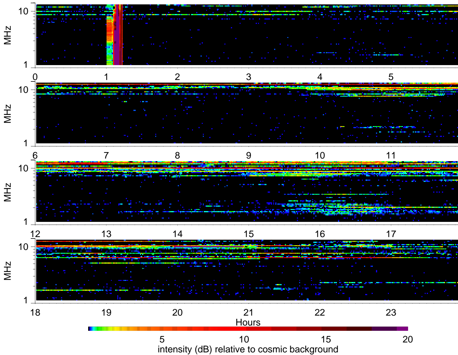
Wind Waves RAD2 receiver: 1996/3/20
