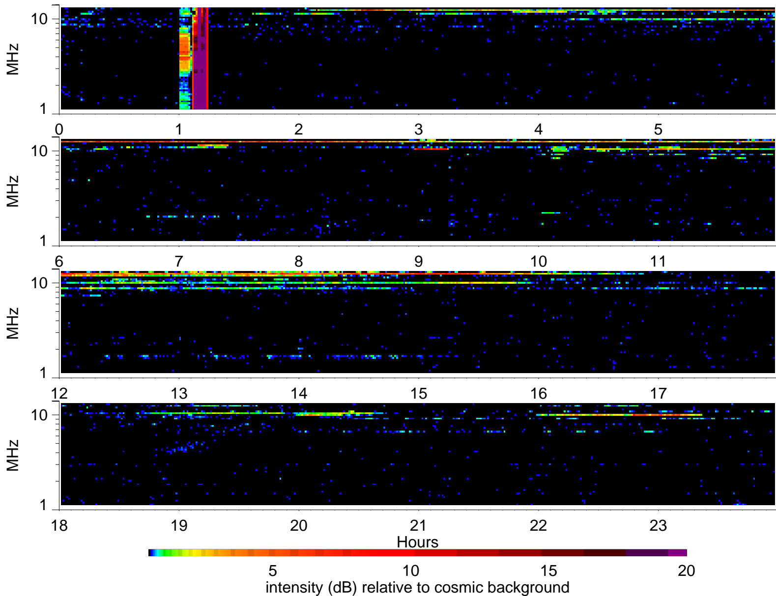
Wind Waves RAD2 receiver: 1996/3/12
