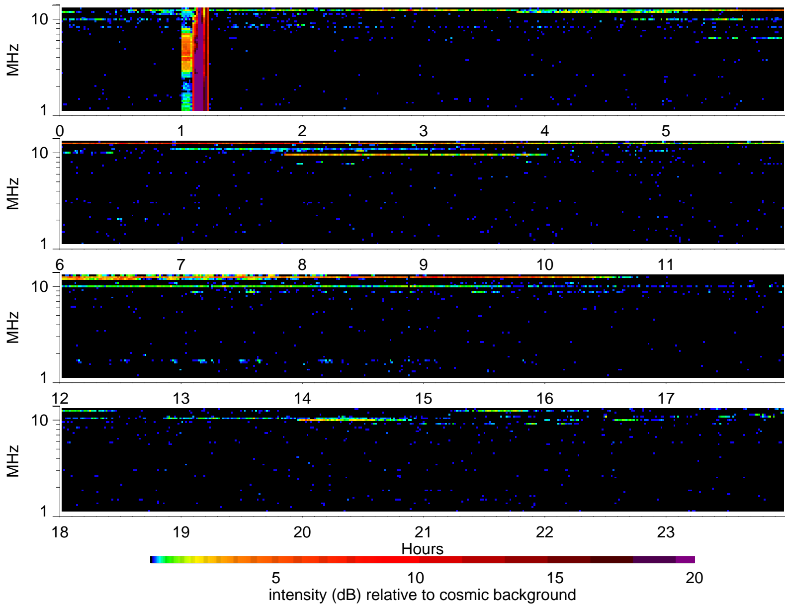
Wind Waves RAD2 receiver: 1996/3/8
