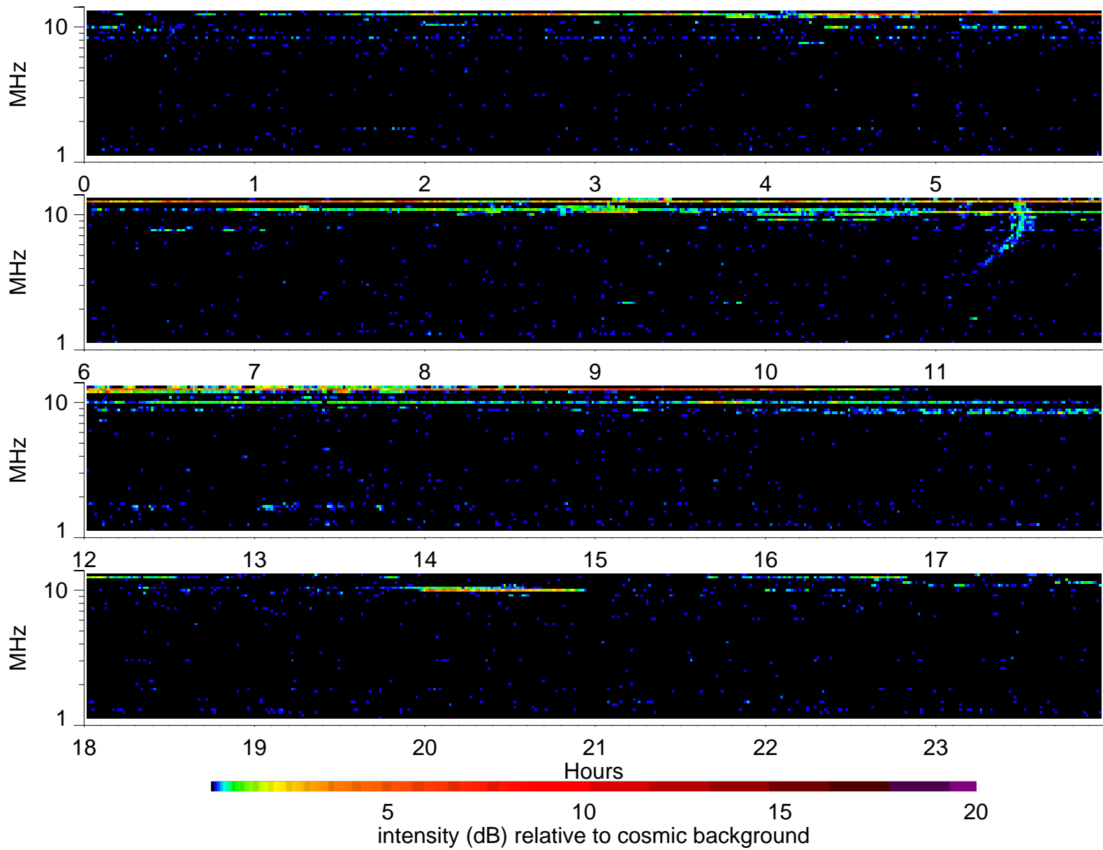
Wind Waves RAD2 receiver: 1996/3/7
