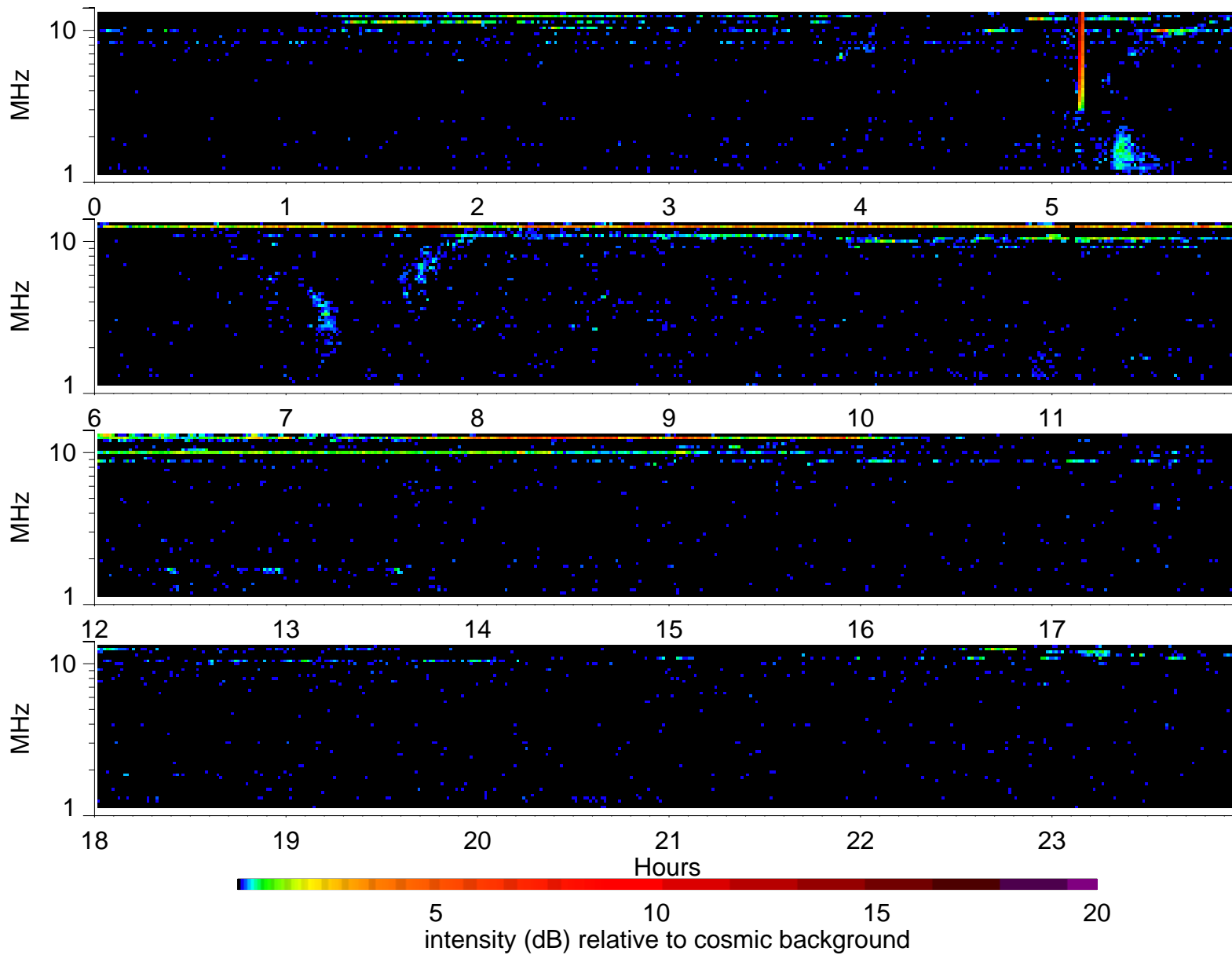
Wind Waves RAD2 receiver: 1996/3/1
