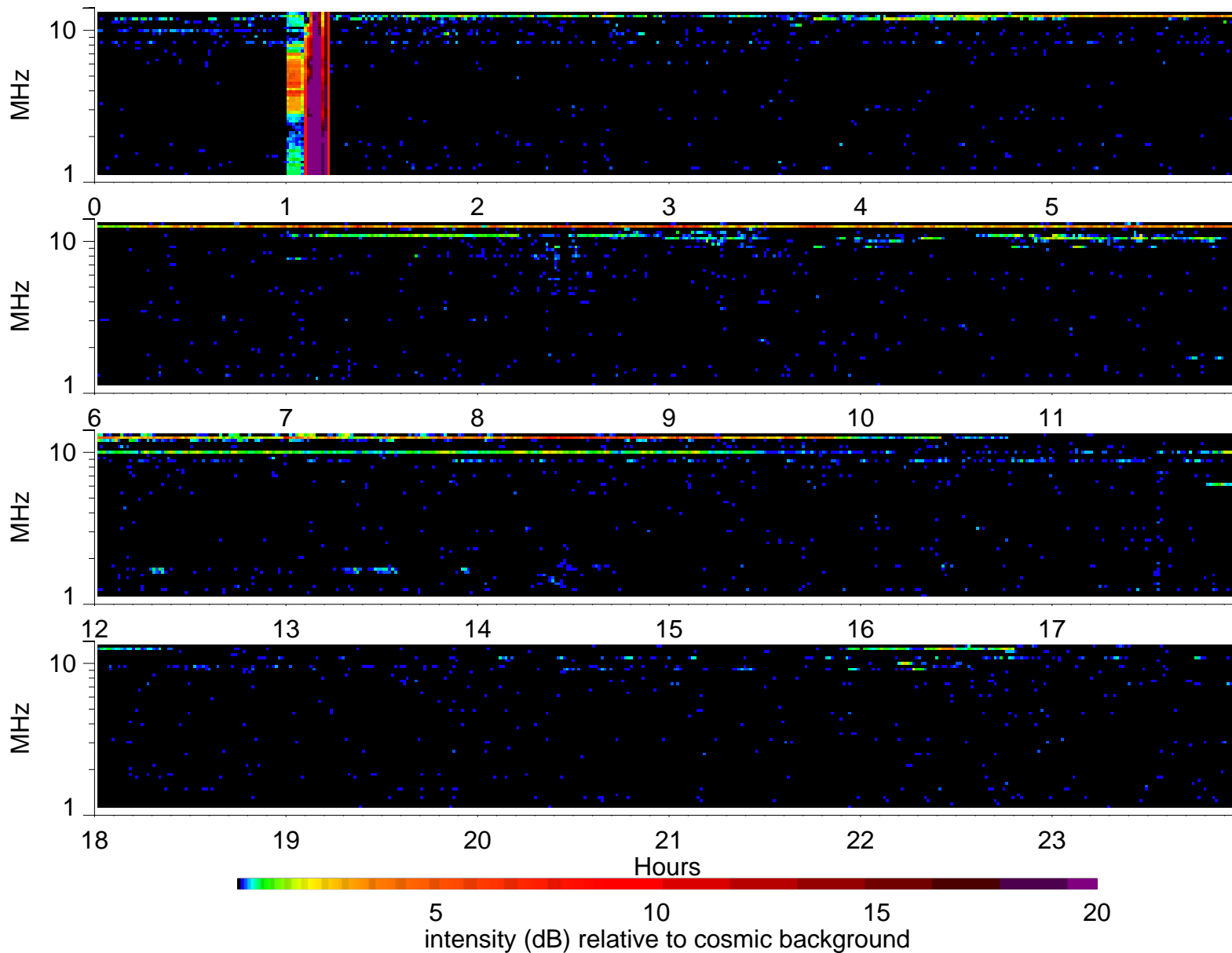
Wind Waves RAD2 receiver: 1996/2/29
