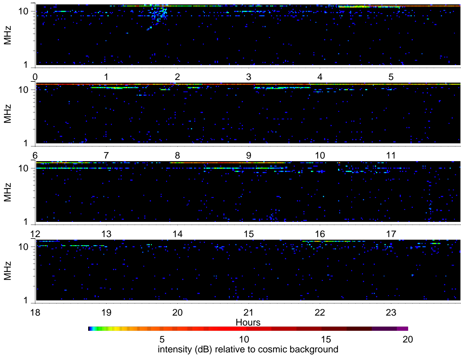
Wind Waves RAD2 receiver: 1996/2/24
