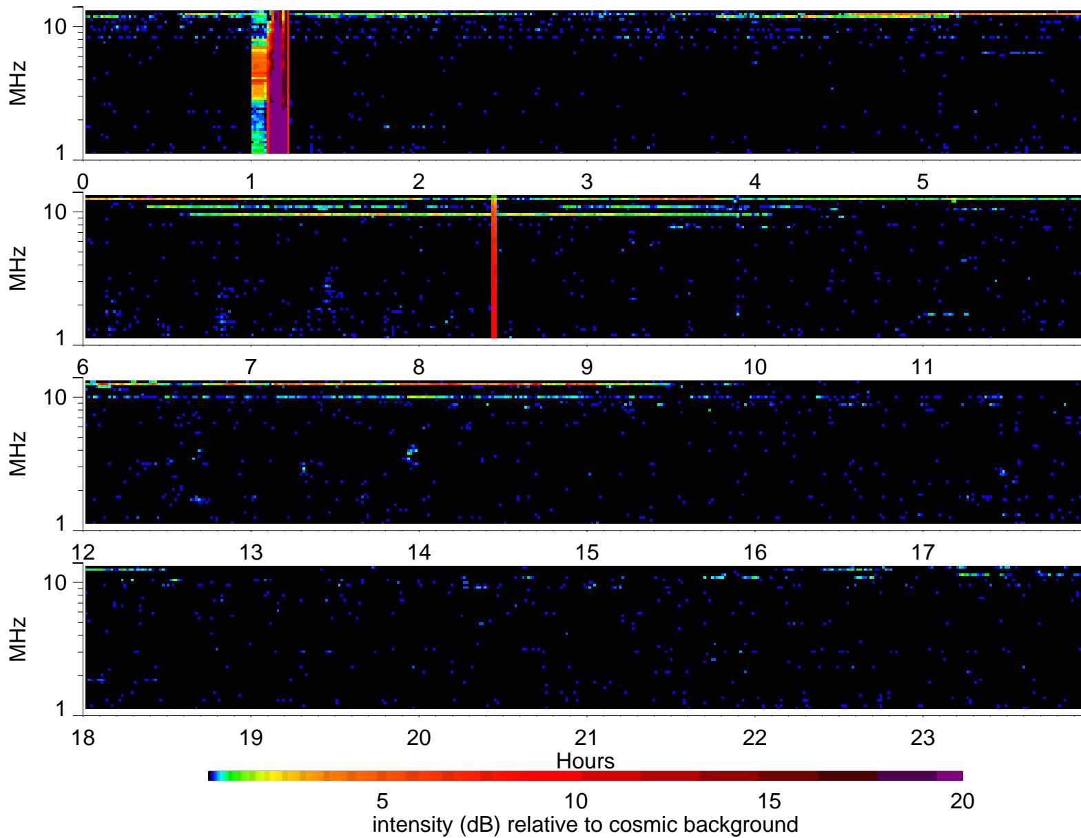
Wind Waves RAD2 receiver: 1996/2/21
