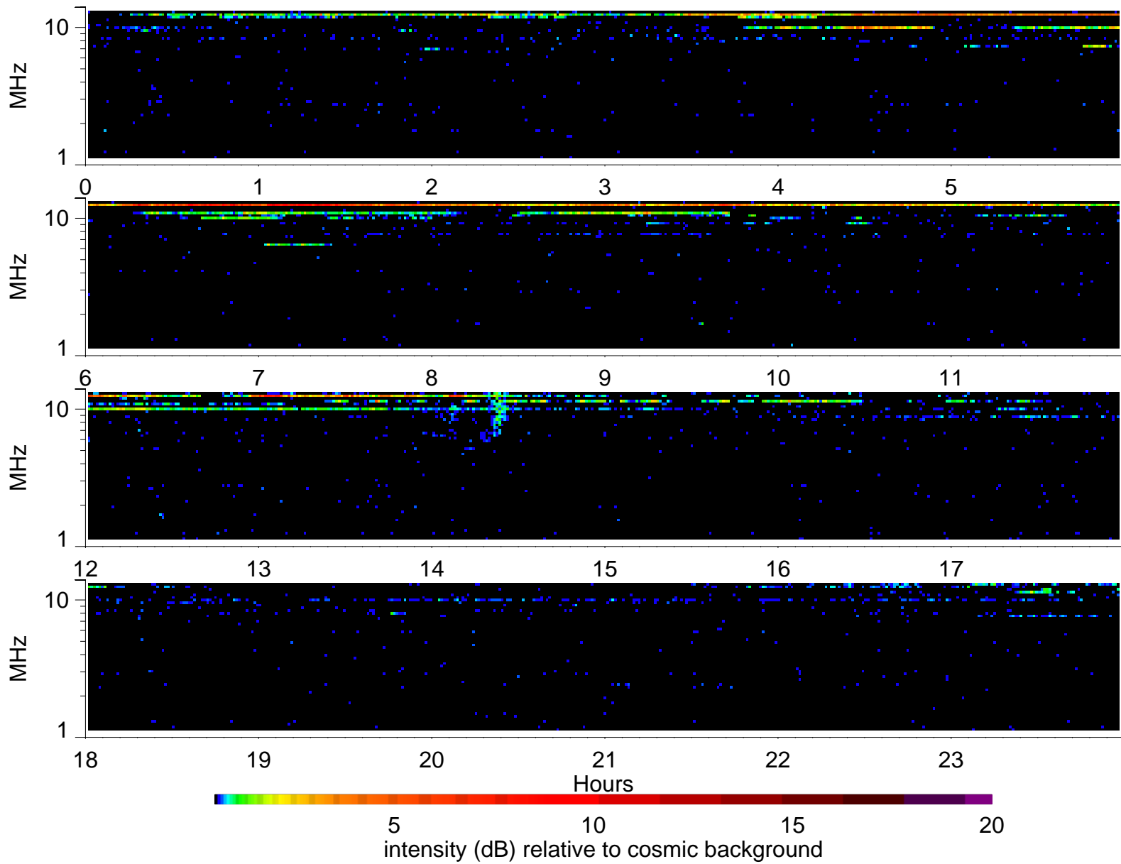
Wind Waves RAD2 receiver: 1996/2/4
