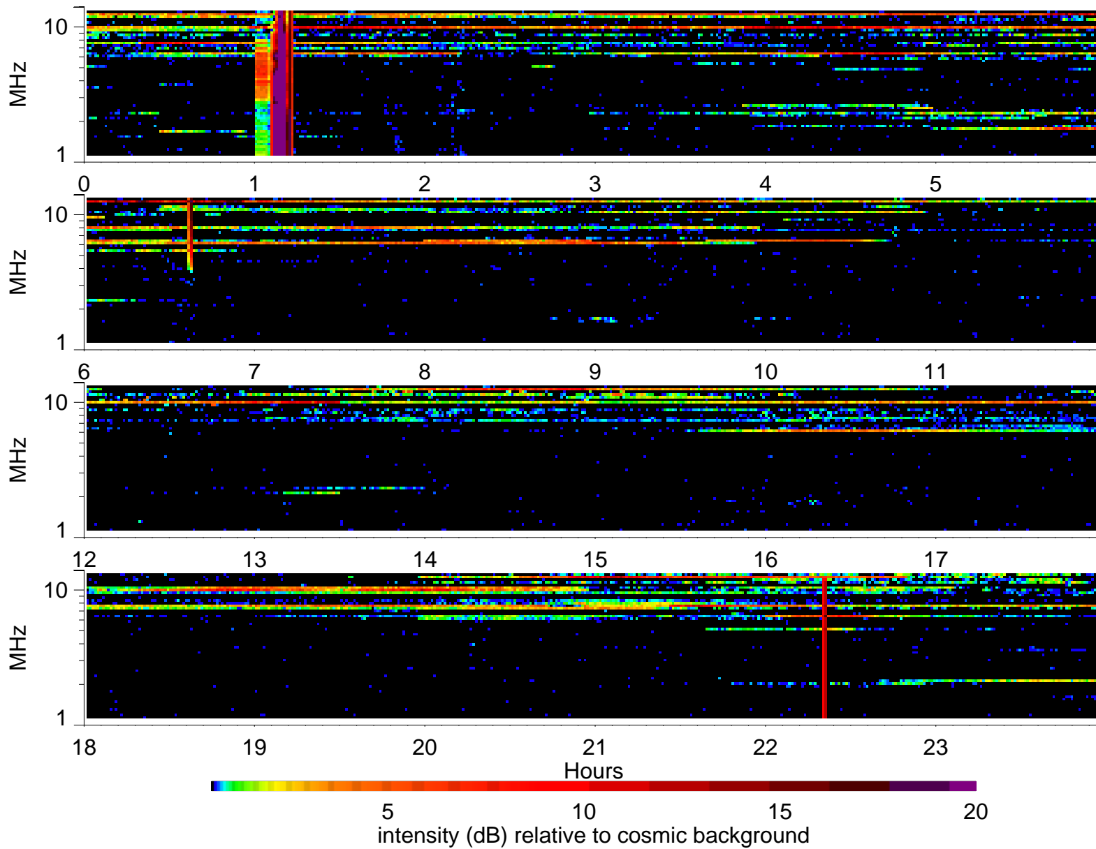
Wind Waves RAD2 receiver: 1996/1/22
