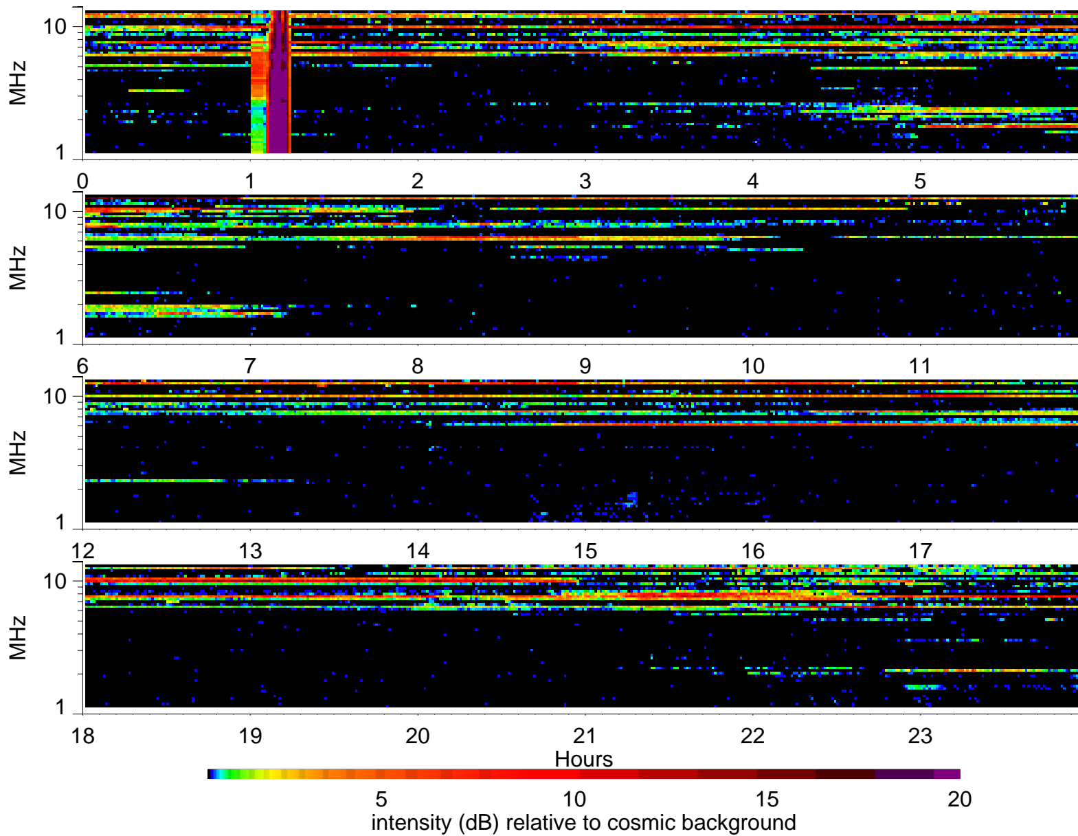
Wind Waves RAD2 receiver: 1996/1/20
