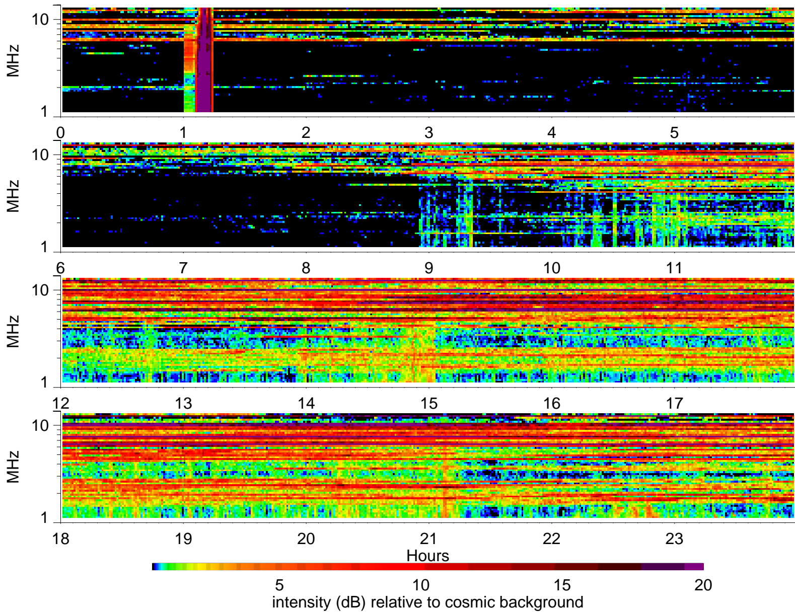
Wind Waves RAD2 receiver: 1996/1/12
