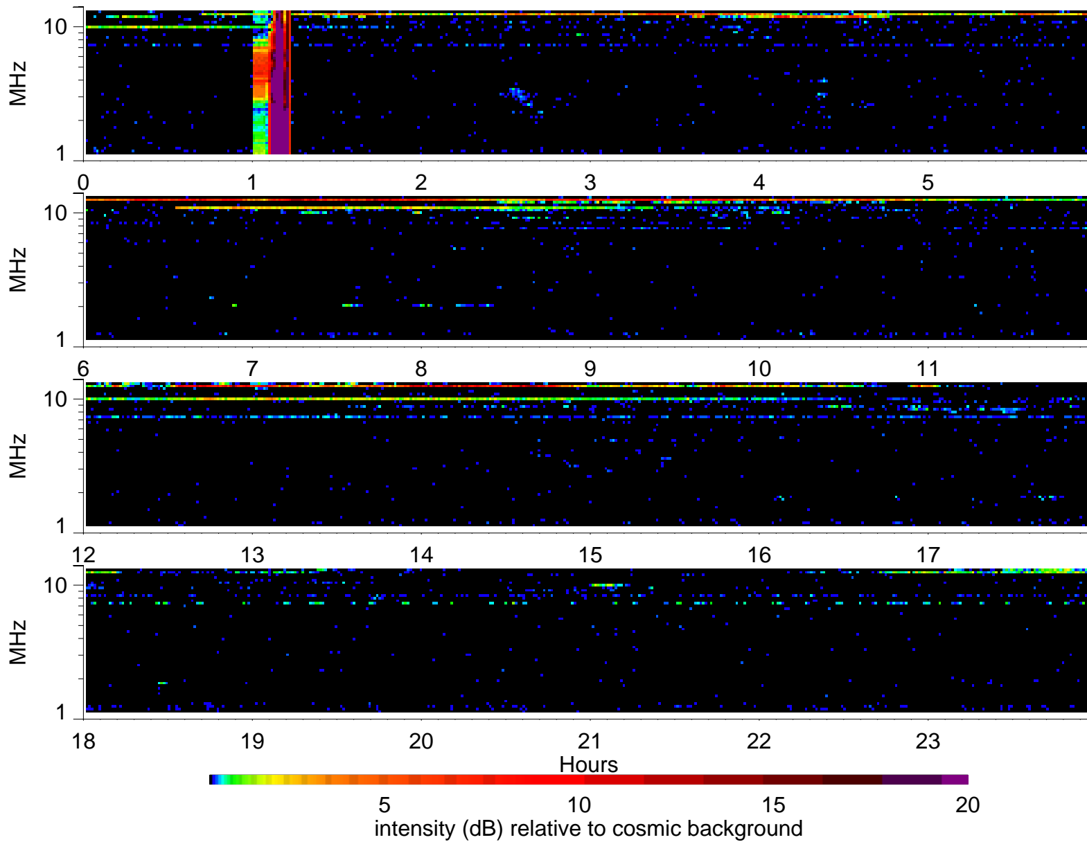
Wind Waves RAD2 receiver: 1996/1/6
