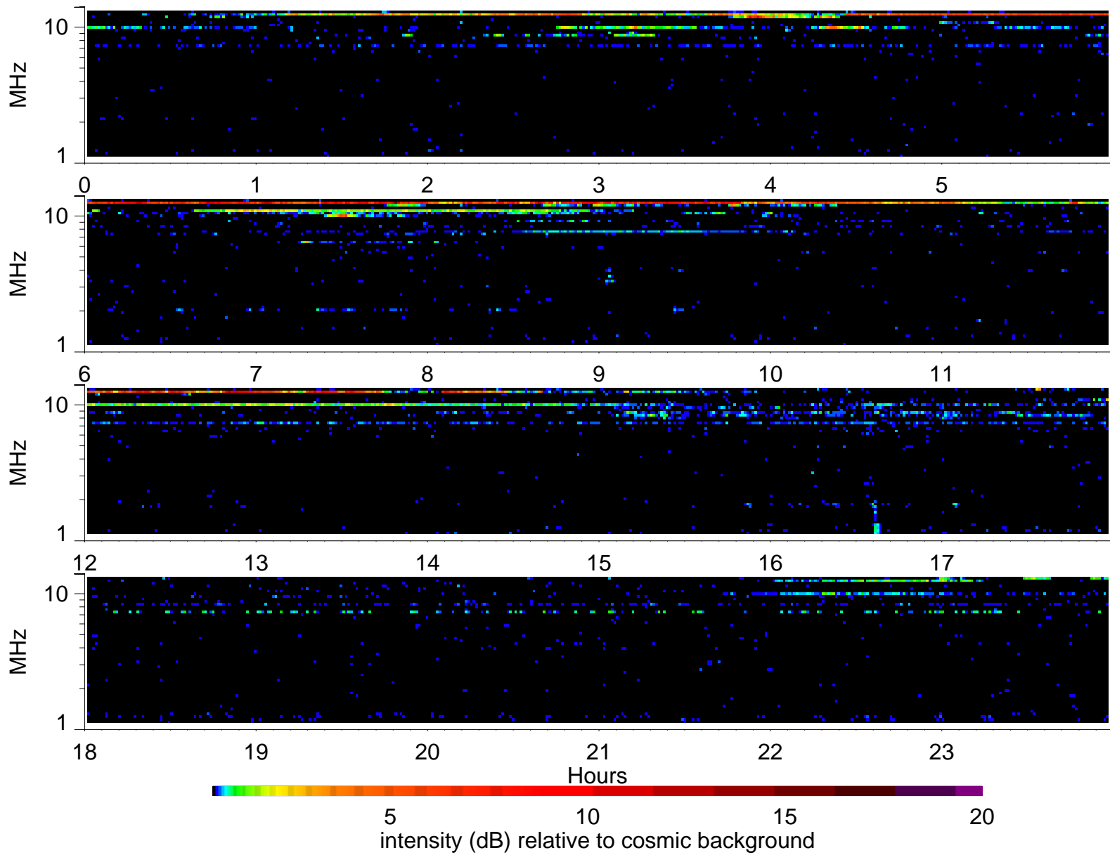
Wind Waves RAD2 receiver: 1996/1/3
