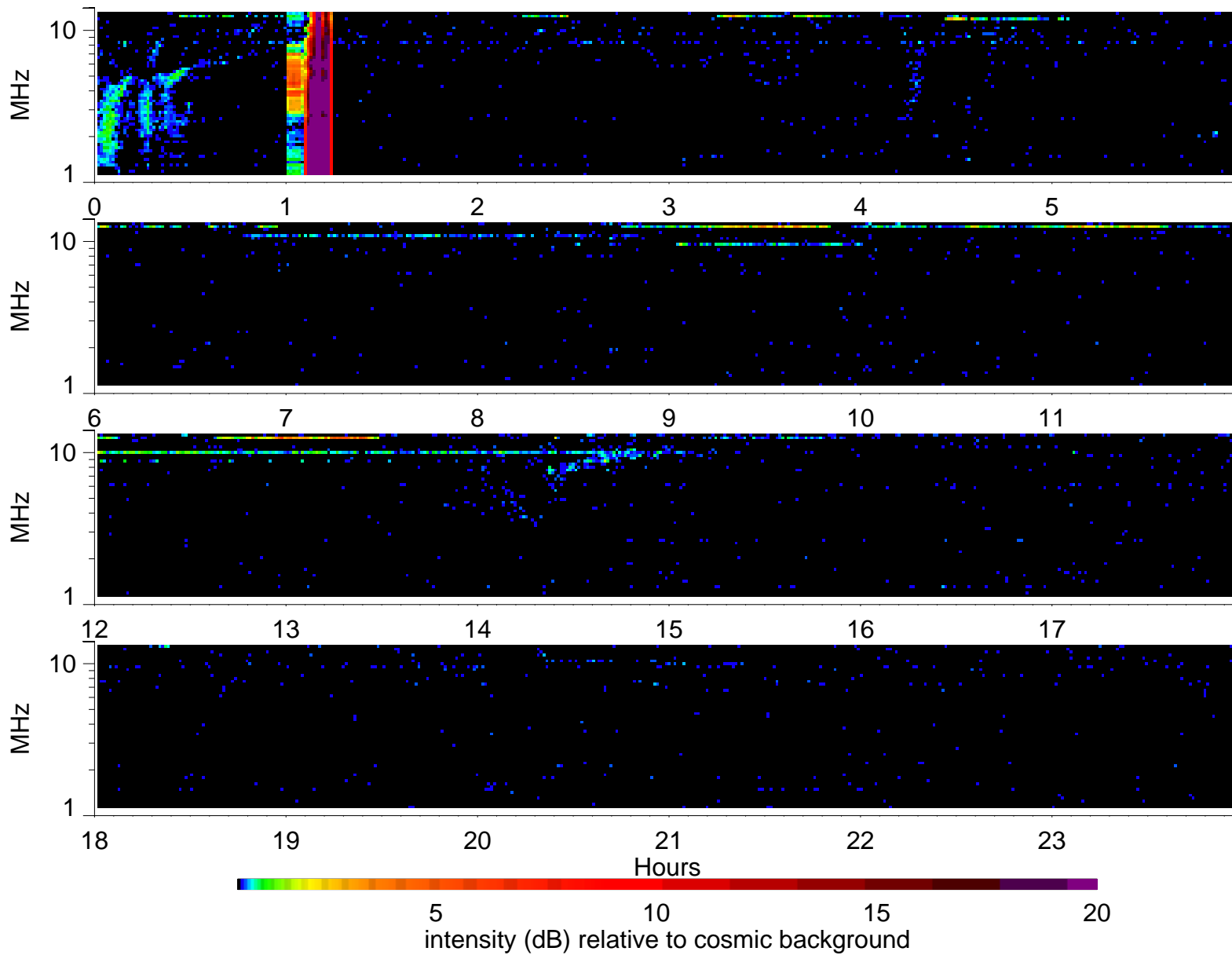
Wind Waves RAD2 receiver: 1995/10/27
