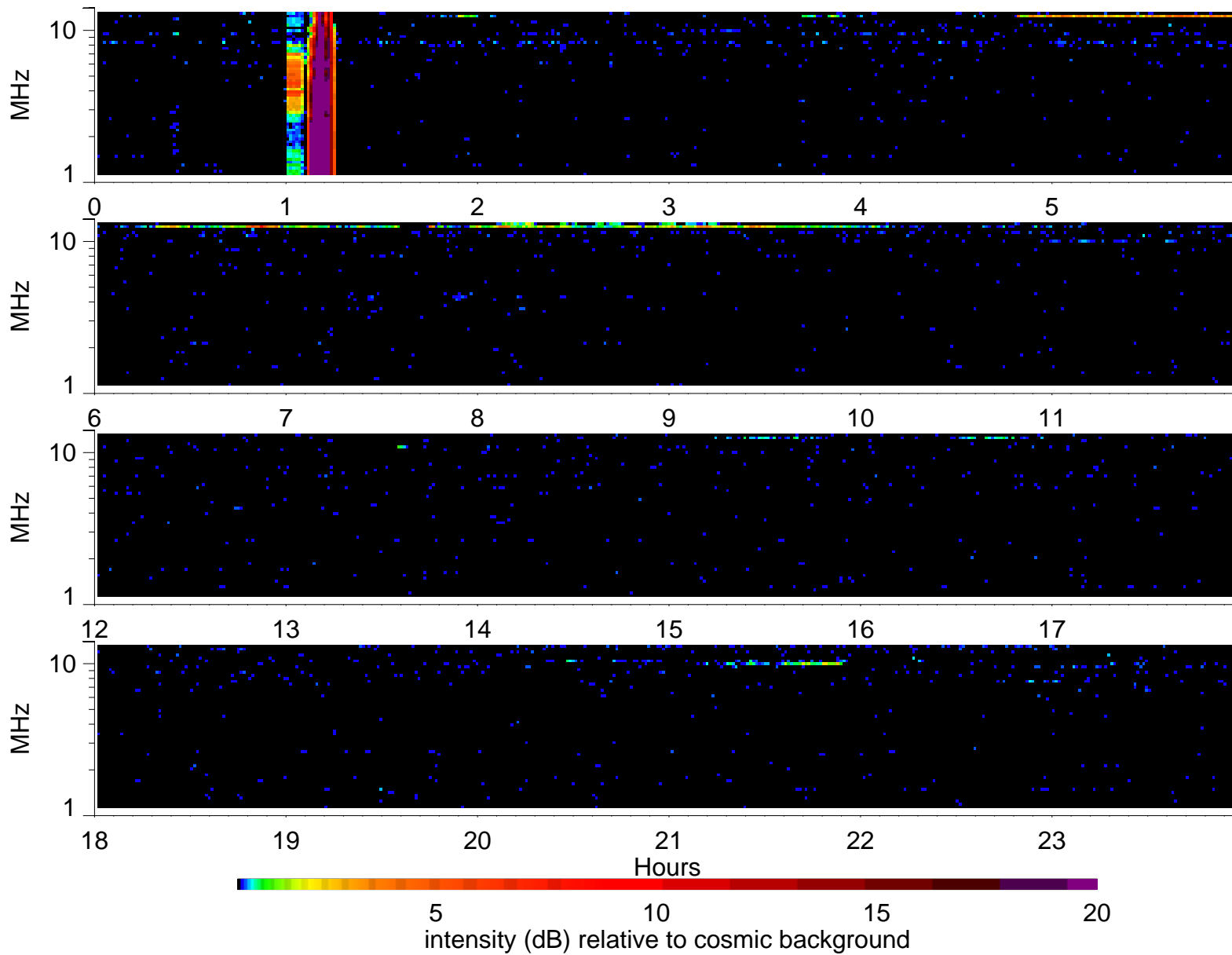
Wind Waves RAD2 receiver: 1995/10/23
