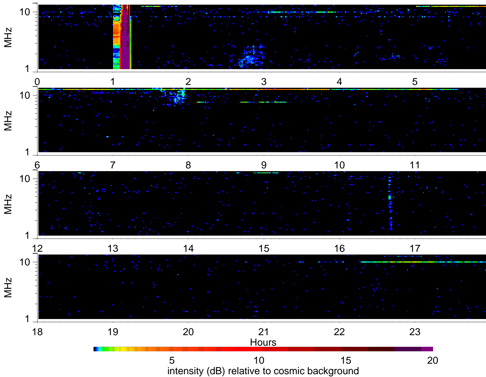
Wind Waves RAD2 receiver: 1995/10/21
