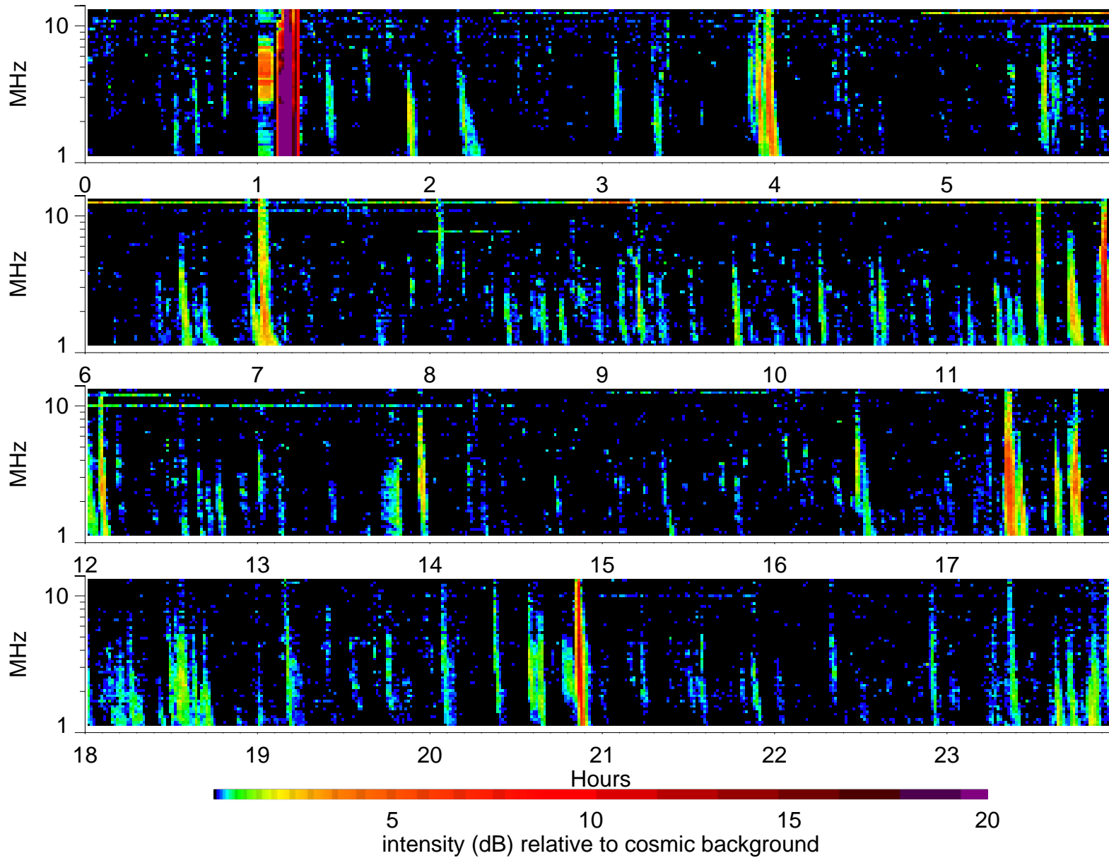
Wind Waves RAD2 receiver: 1995/10/17
