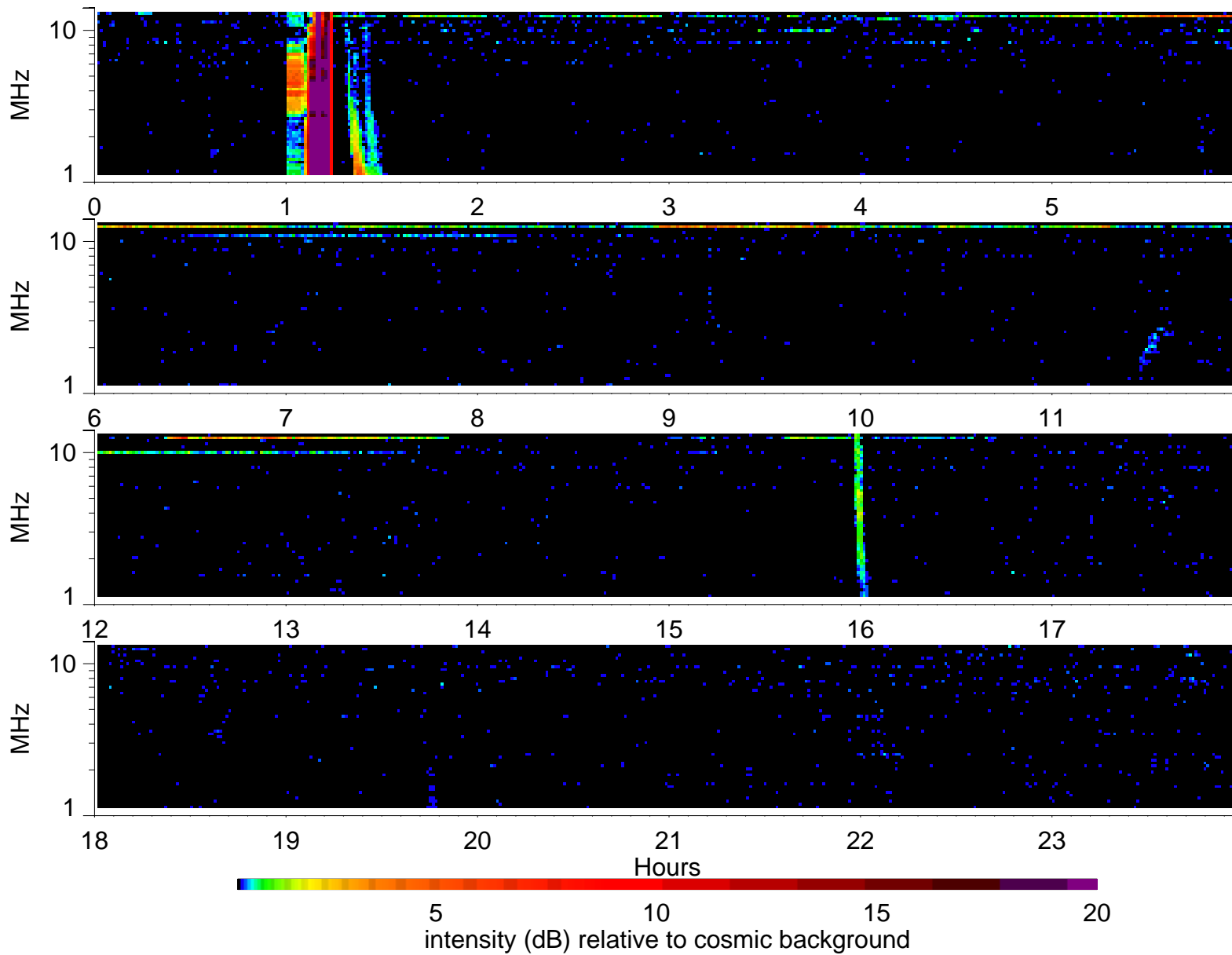
Wind Waves RAD2 receiver: 1995/10/11
