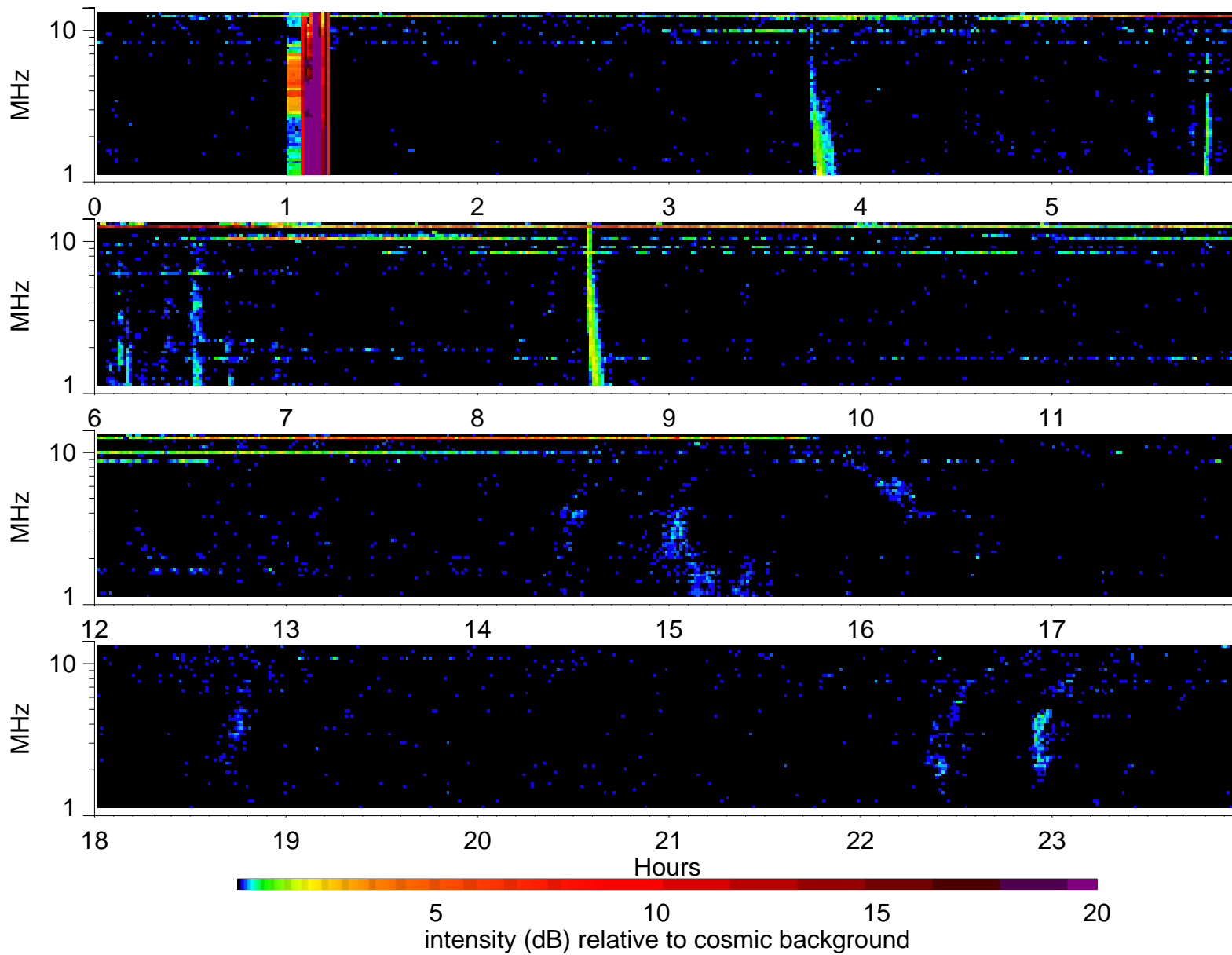
Wind Waves RAD2 receiver: 1995/10/7
