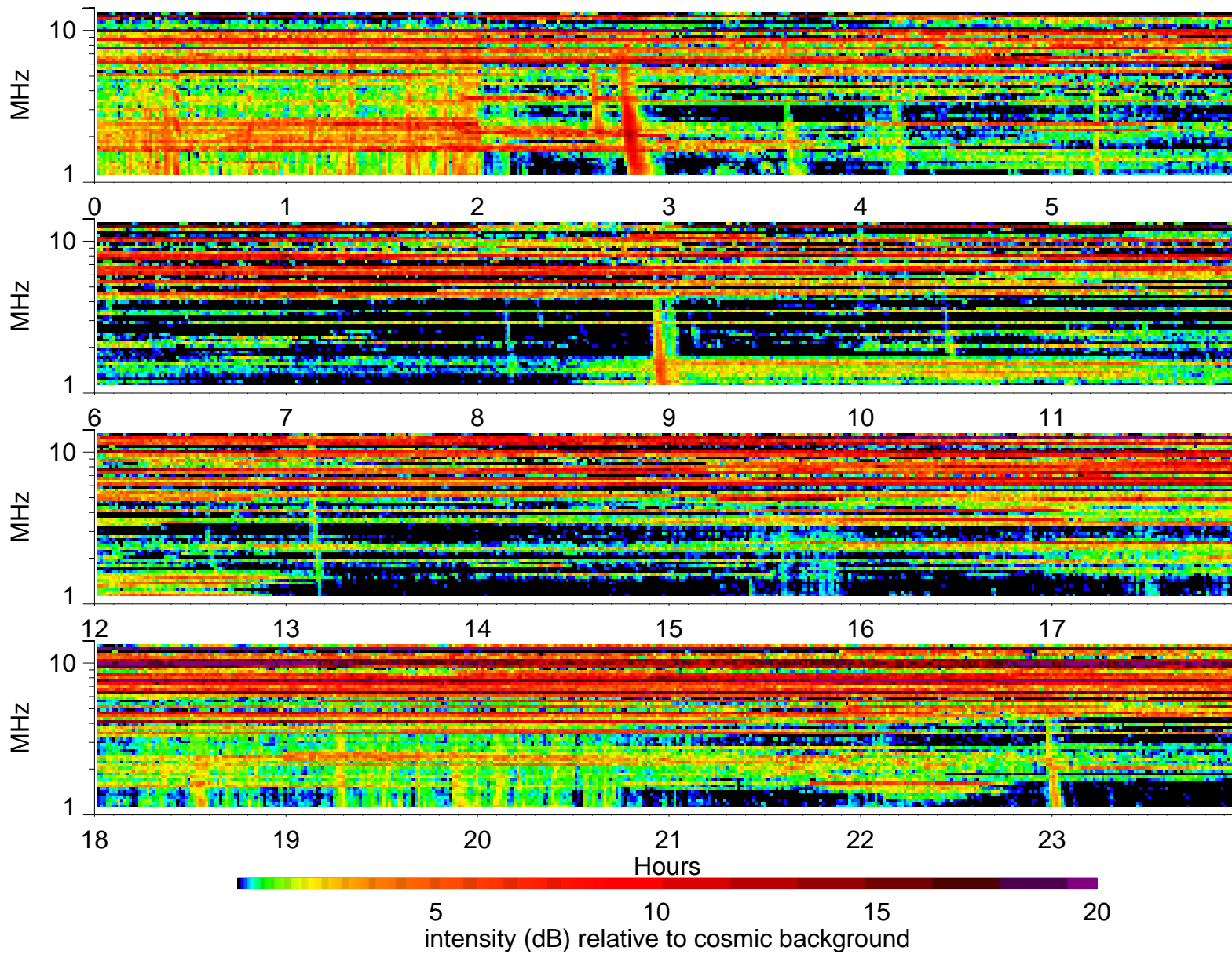
Wind Waves RAD2 receiver: 1995/9/17
