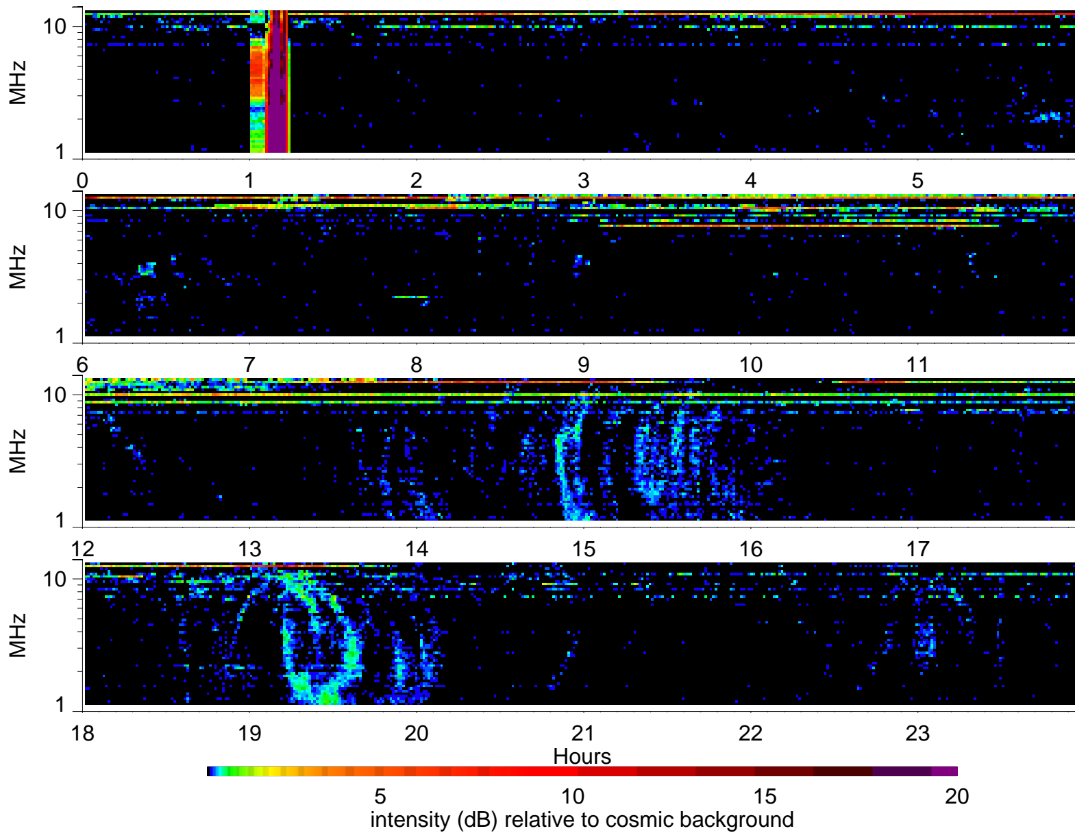
Wind Waves RAD2 receiver: 1995/9/5
