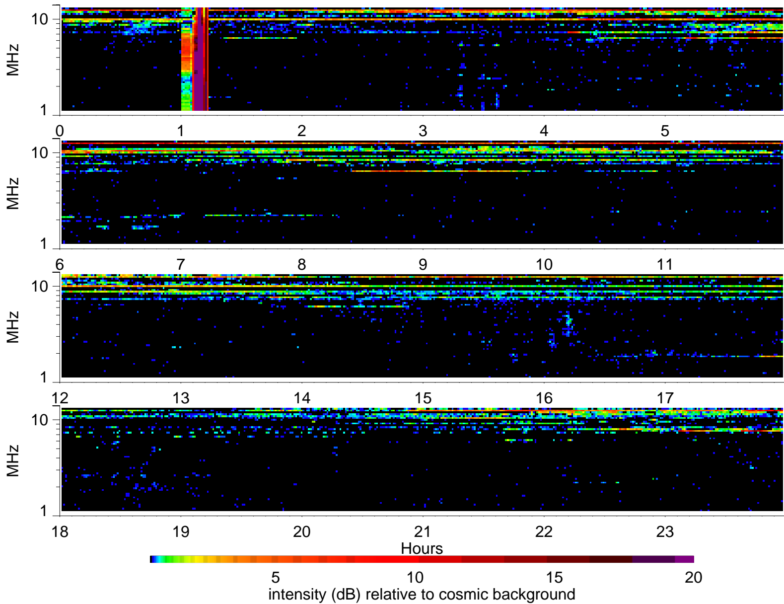
Wind Waves RAD2 receiver: 1995/8/26
