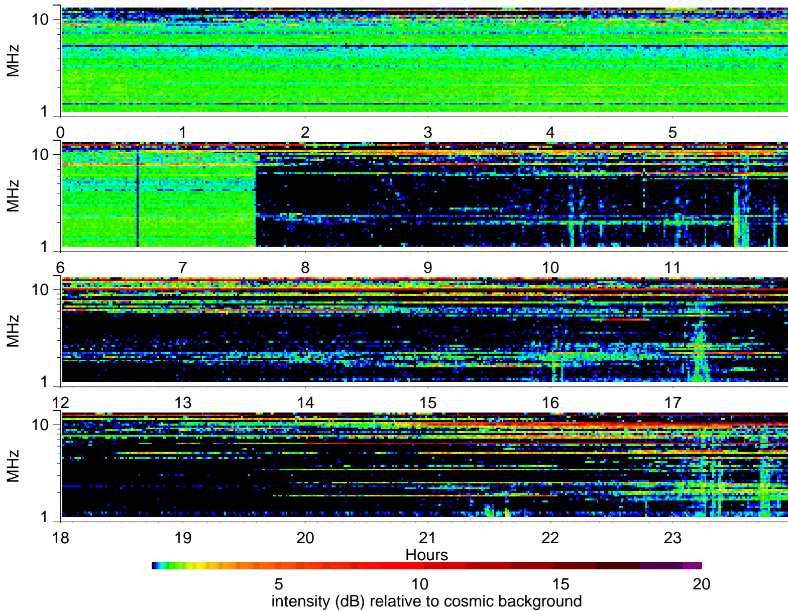
Wind Waves RAD2 receiver: 1995/8/19
