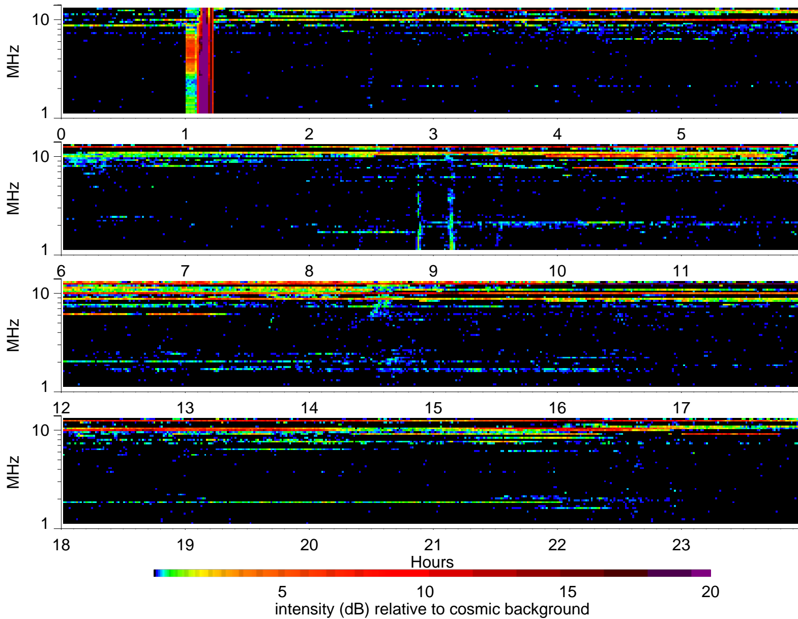
Wind Waves RAD2 receiver: 1995/8/18
