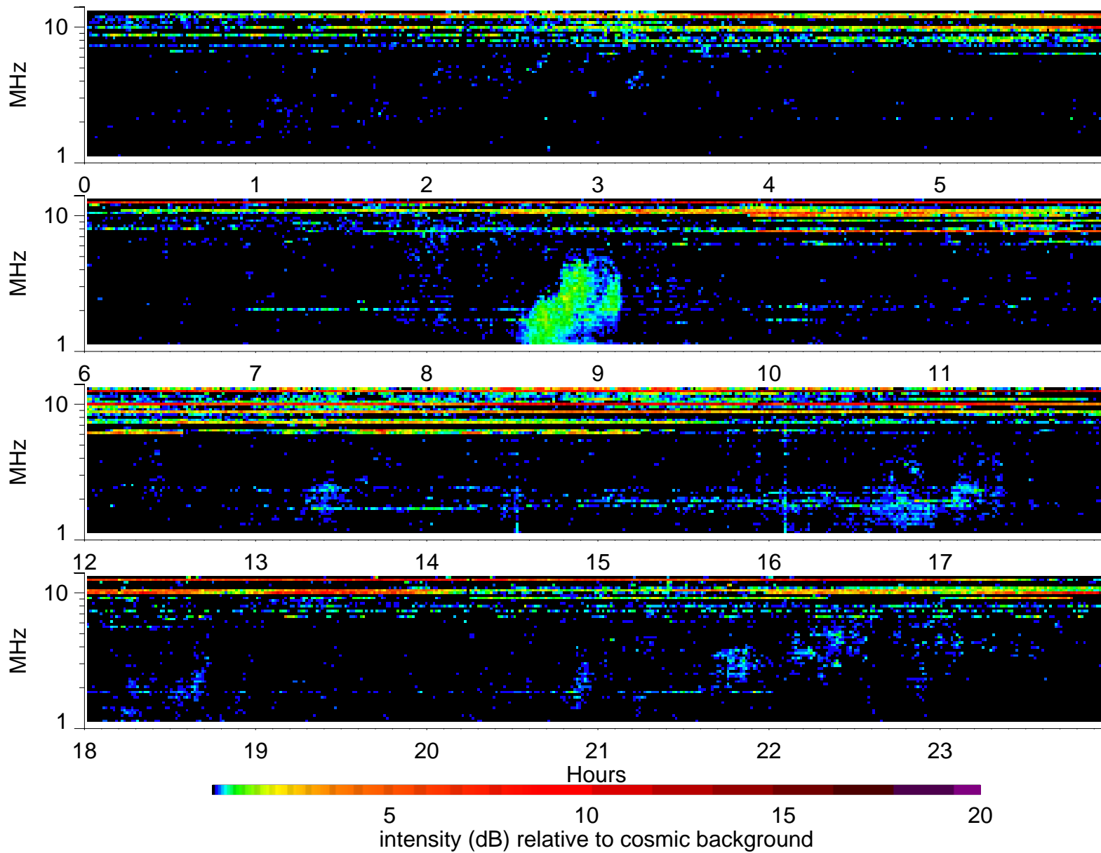
Wind Waves RAD2 receiver: 1995/7/30
