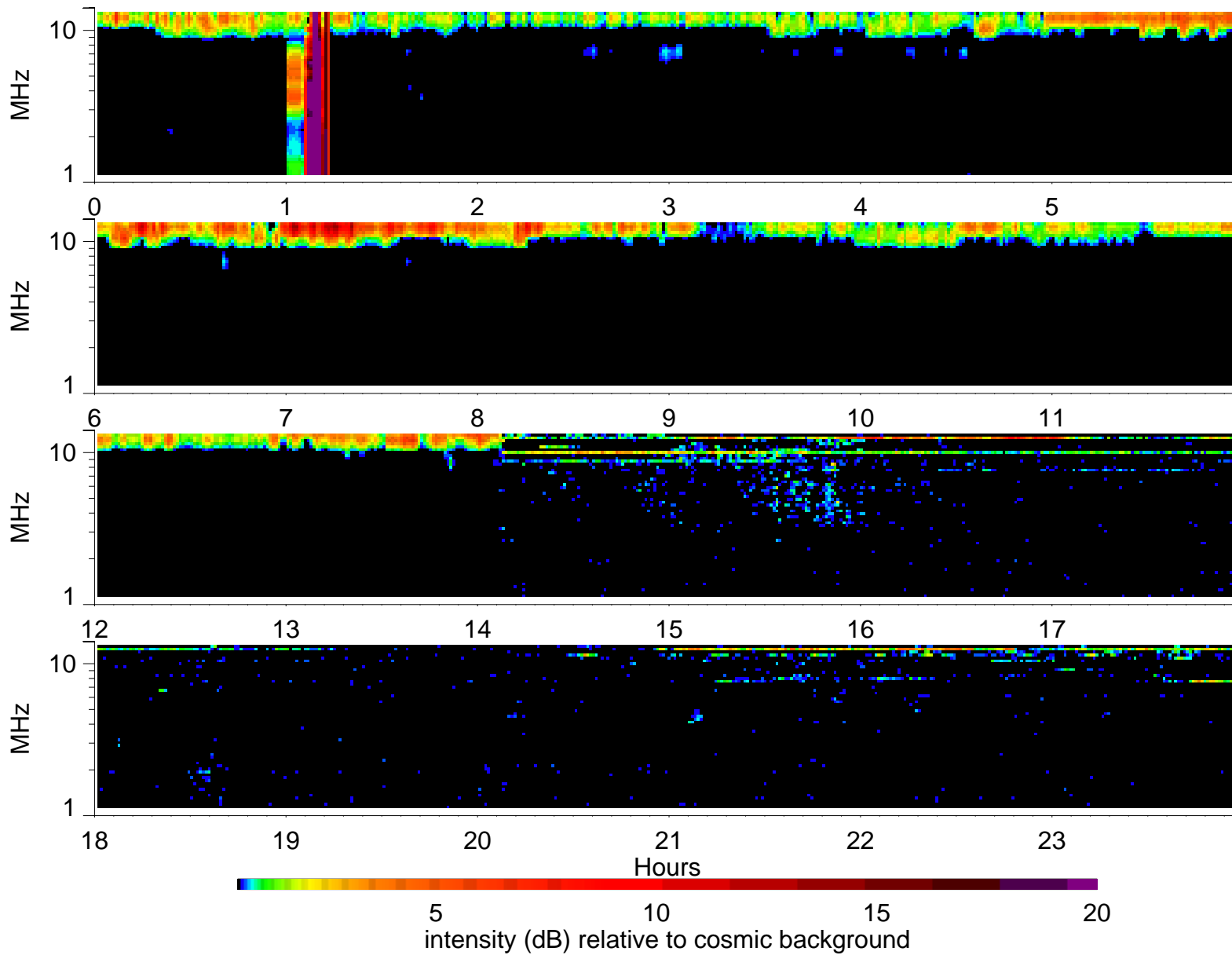
Wind Waves RAD2 receiver: 1995/7/11
