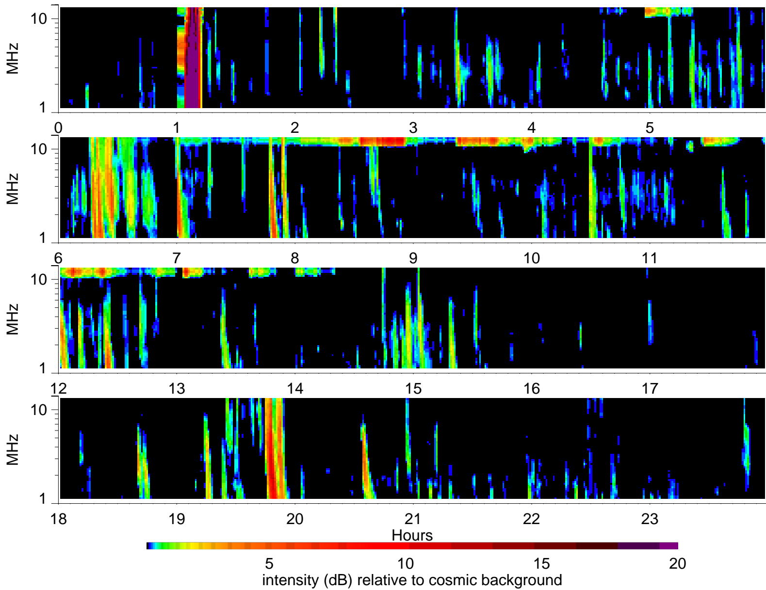
Wind Waves RAD2 receiver: 1995/3/3
