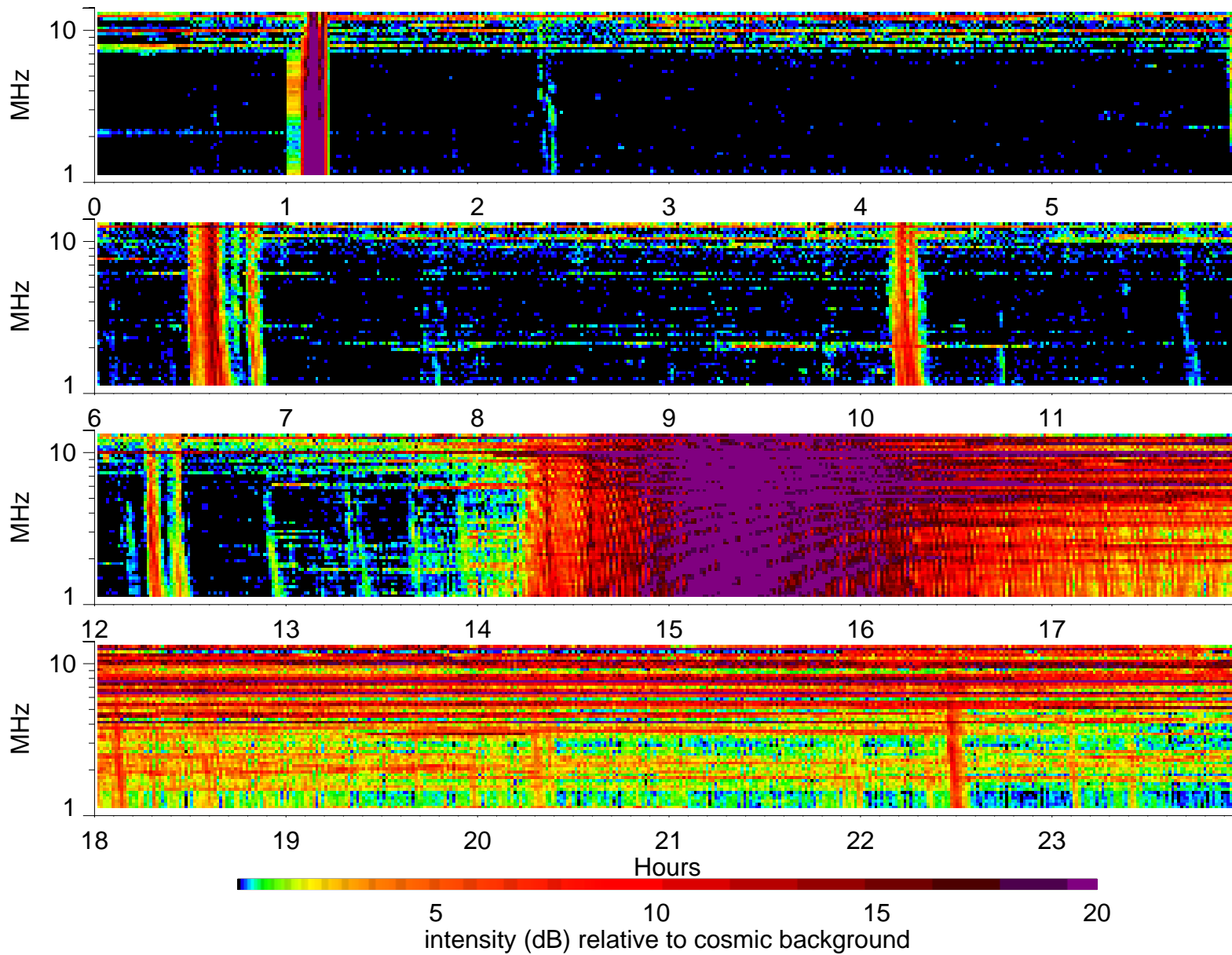
Wind Waves RAD2 receiver: 1994/12/24
