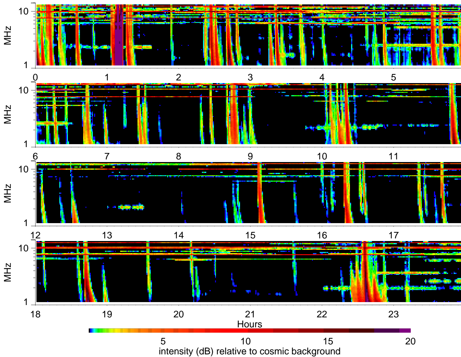
Wind Waves RAD2 receiver: 1994/12/22
