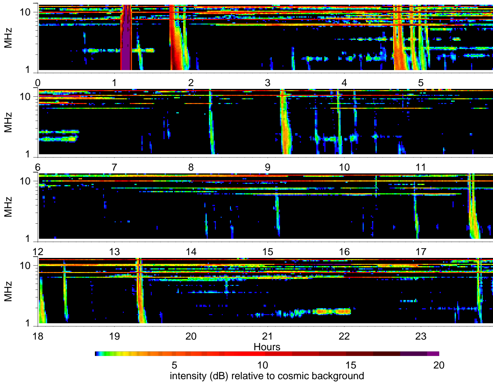
Wind Waves RAD2 receiver: 1994/12/19
