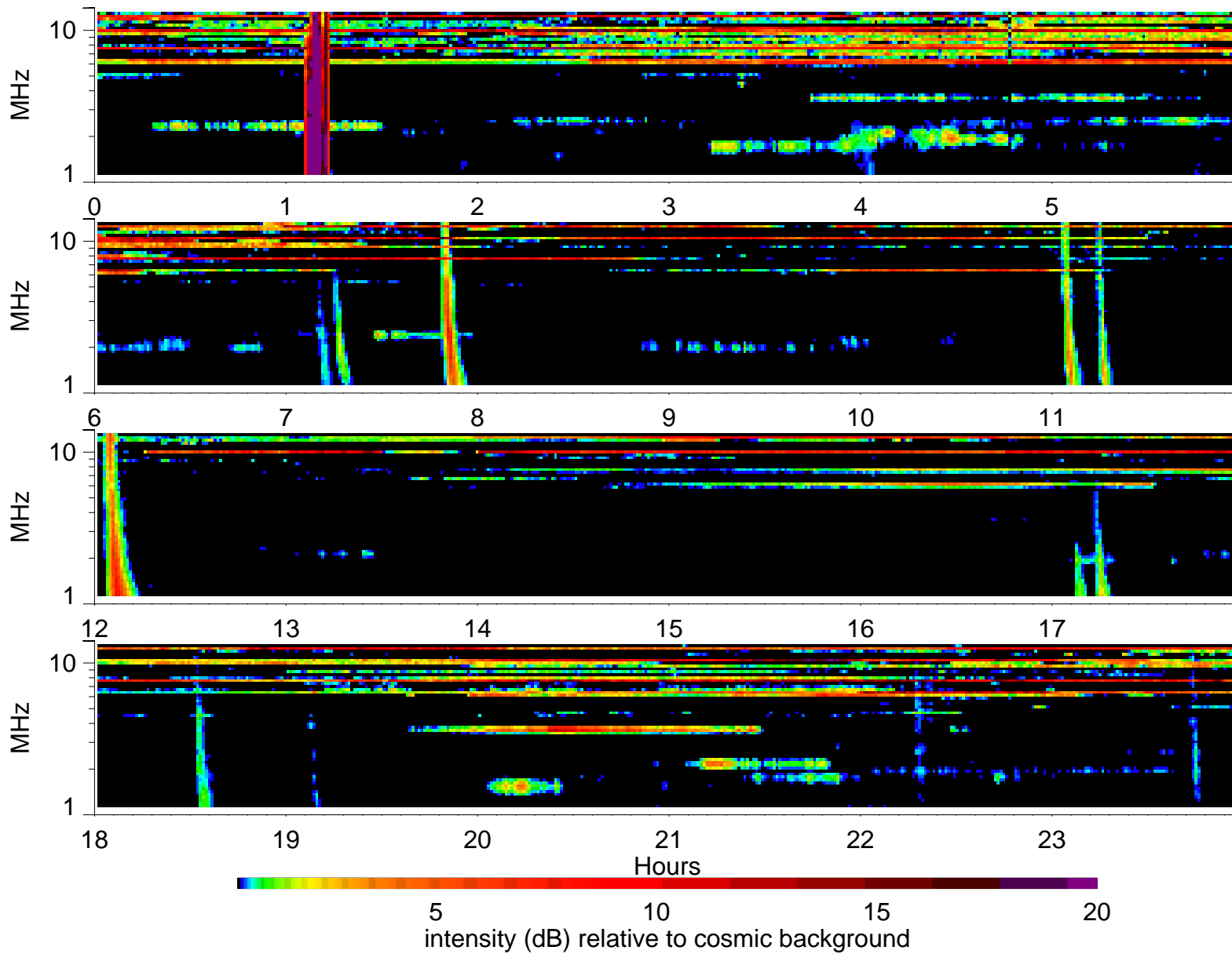
Wind Waves RAD2 receiver: 1994/12/16
