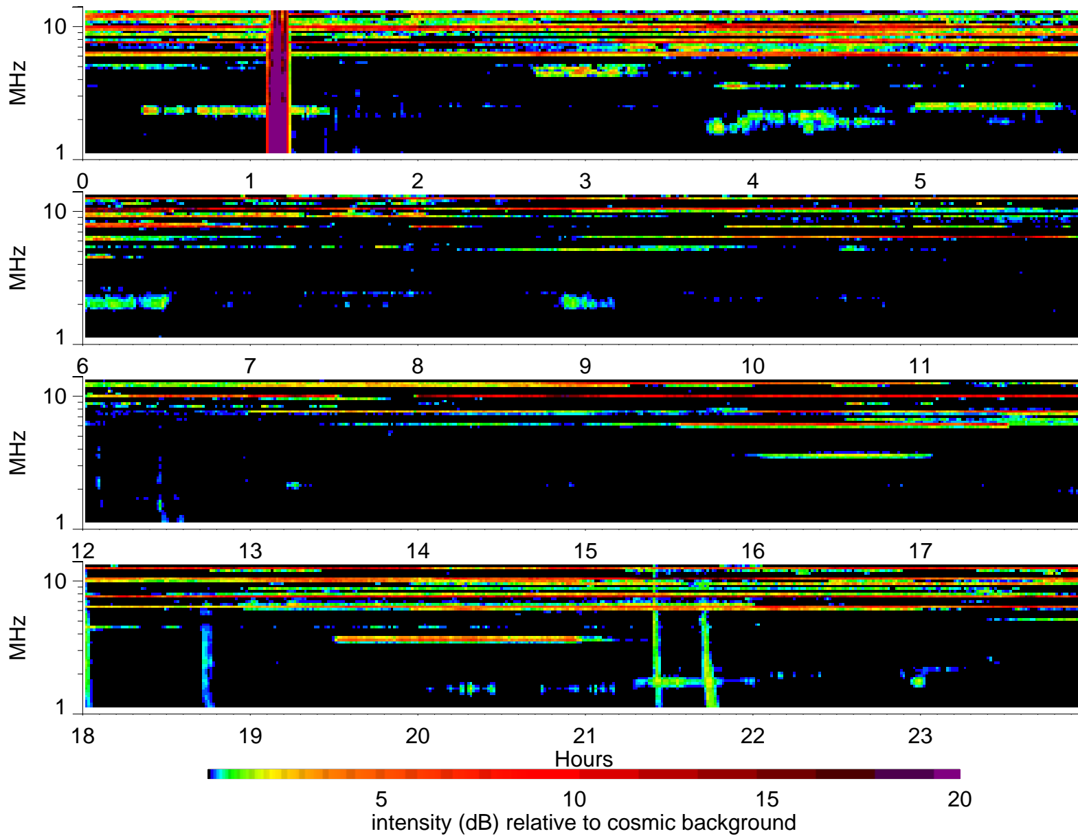
Wind Waves RAD2 receiver: 1994/12/15
