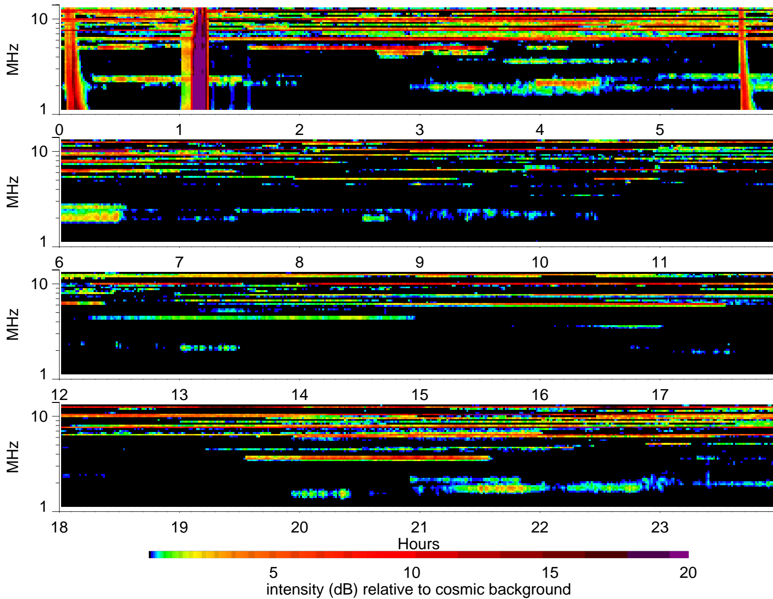
Wind Waves RAD2 receiver: 1994/12/14
