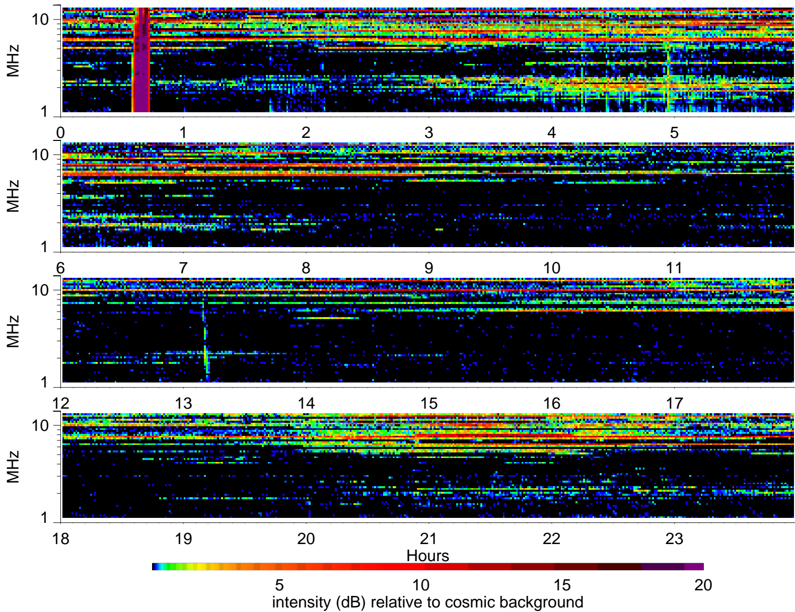
Wind Waves RAD2 receiver: 1994/12/3
