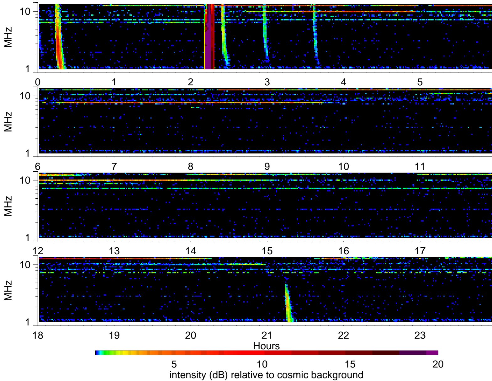
Wind Waves RAD2 receiver: 1994/11/28
