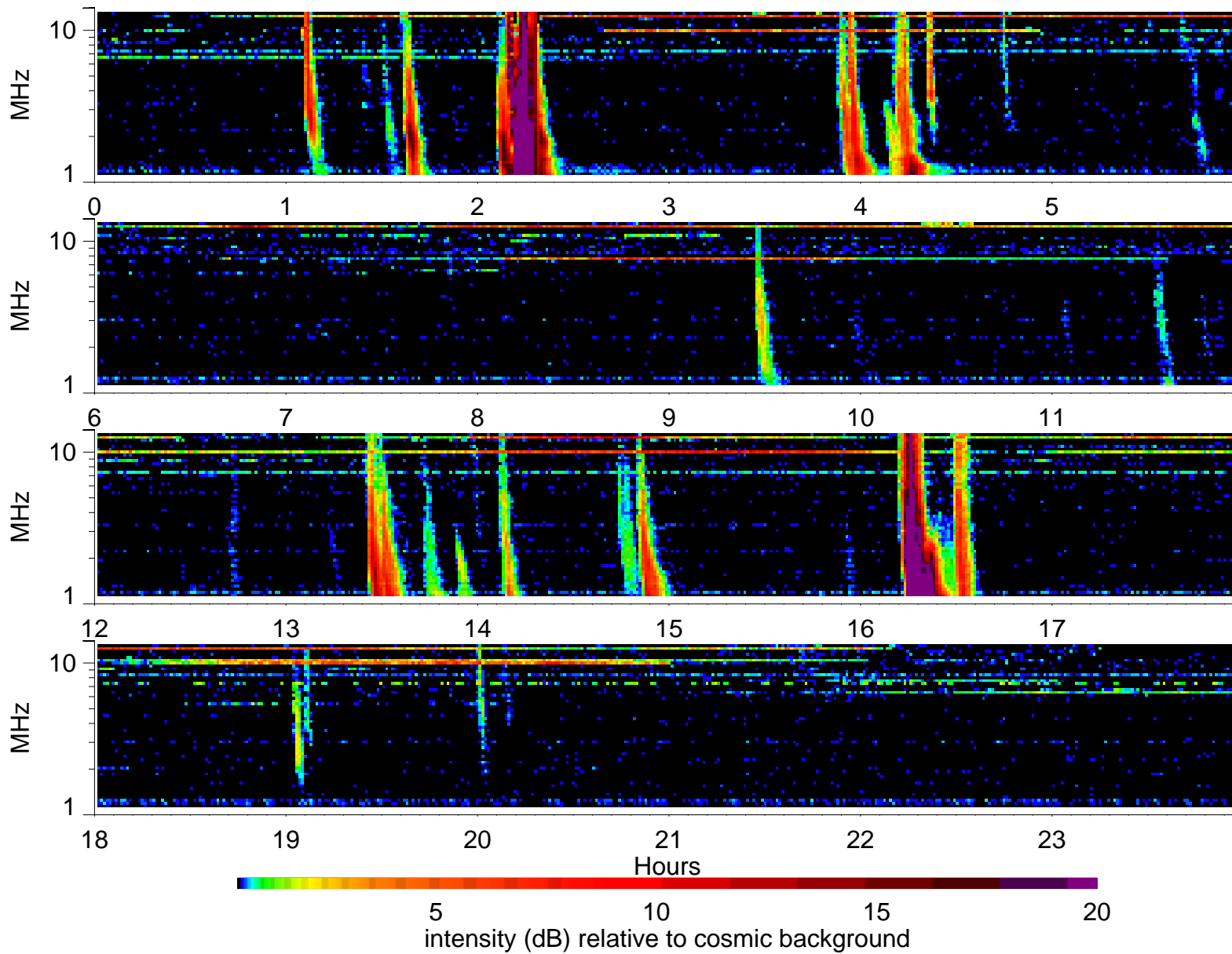
Wind Waves RAD2 receiver: 1994/11/27
