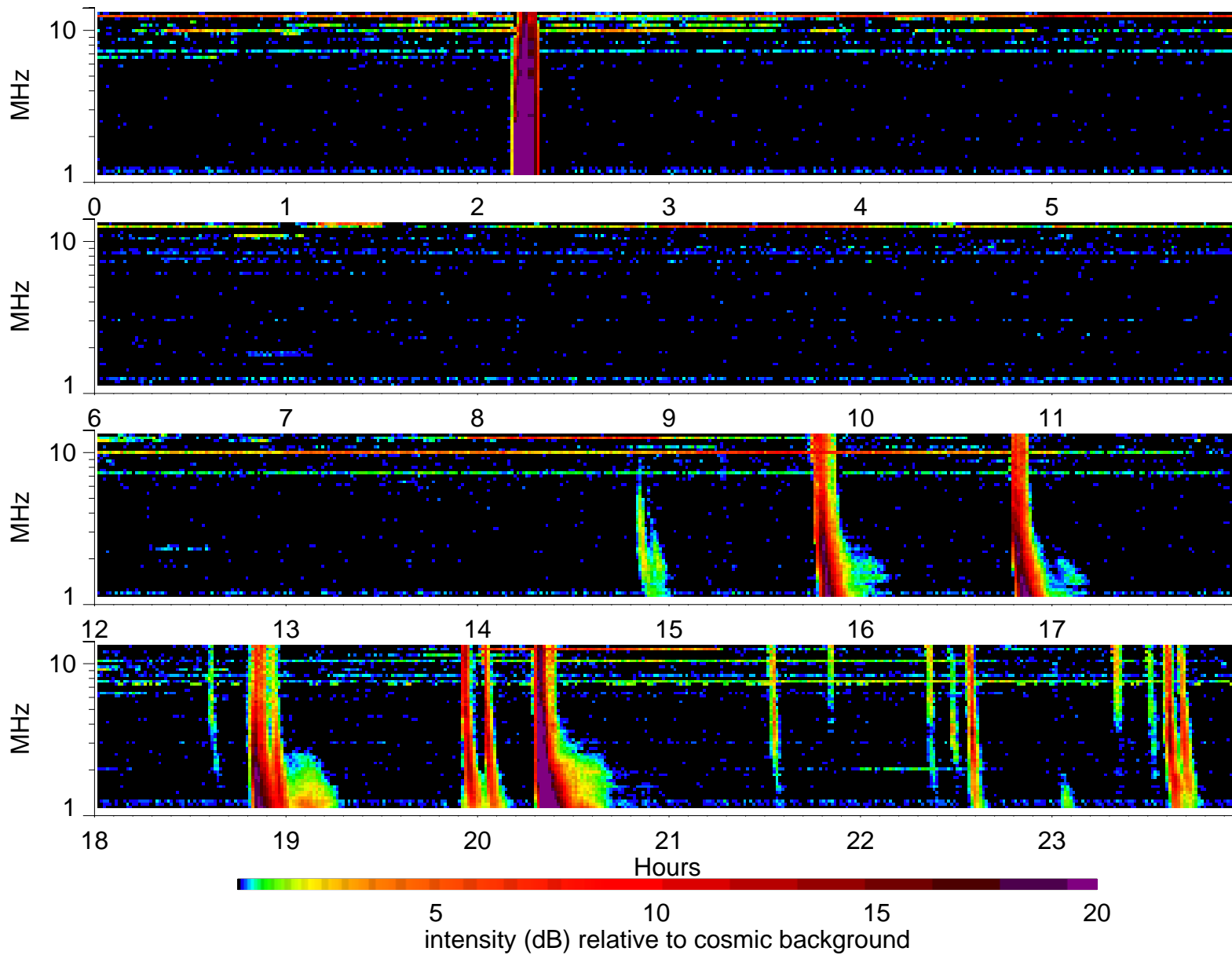
Wind Waves RAD2 receiver: 1994/11/26
