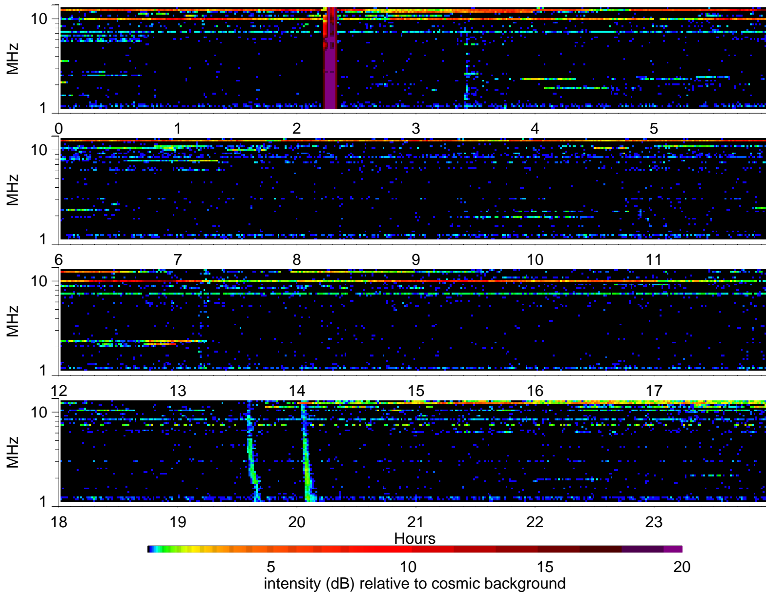
Wind Waves RAD2 receiver: 1994/11/23
