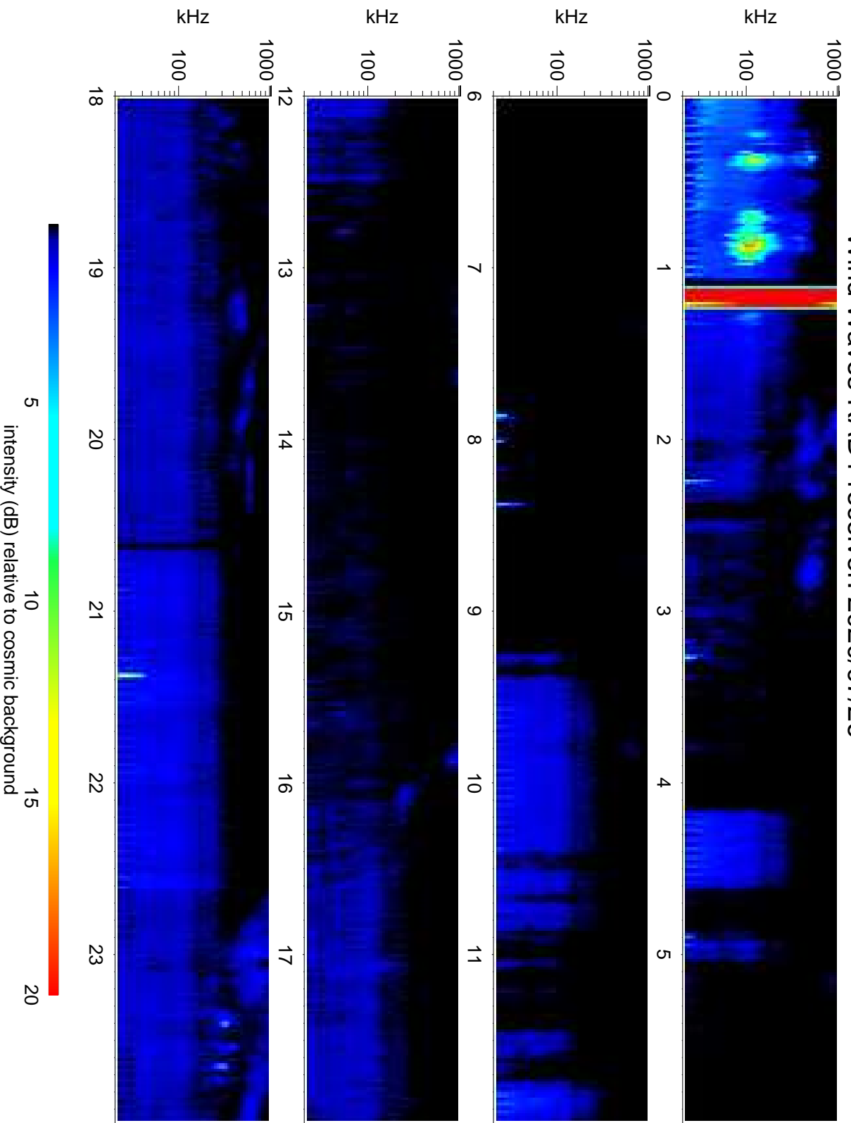
Wind Waves RAD1 receiver: 2020/07/26
