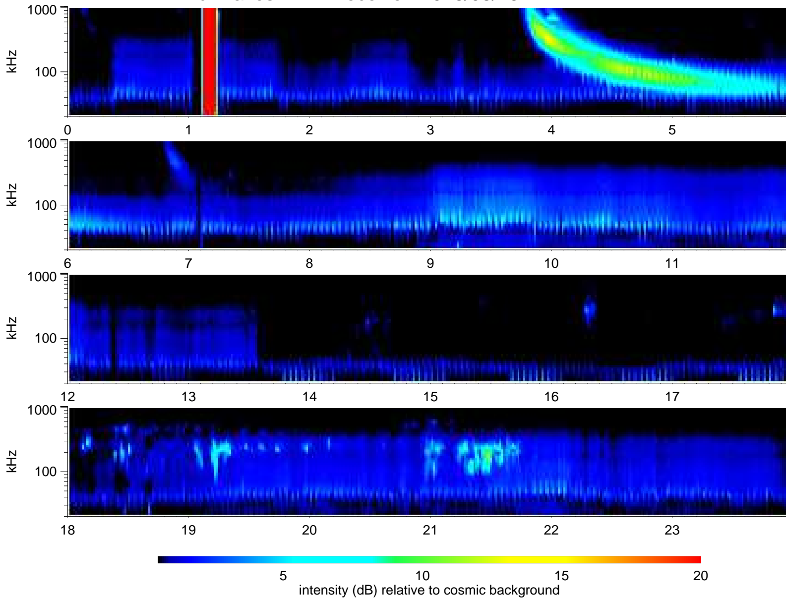
Wind Waves RAD1 receiver: 2016/08/29
