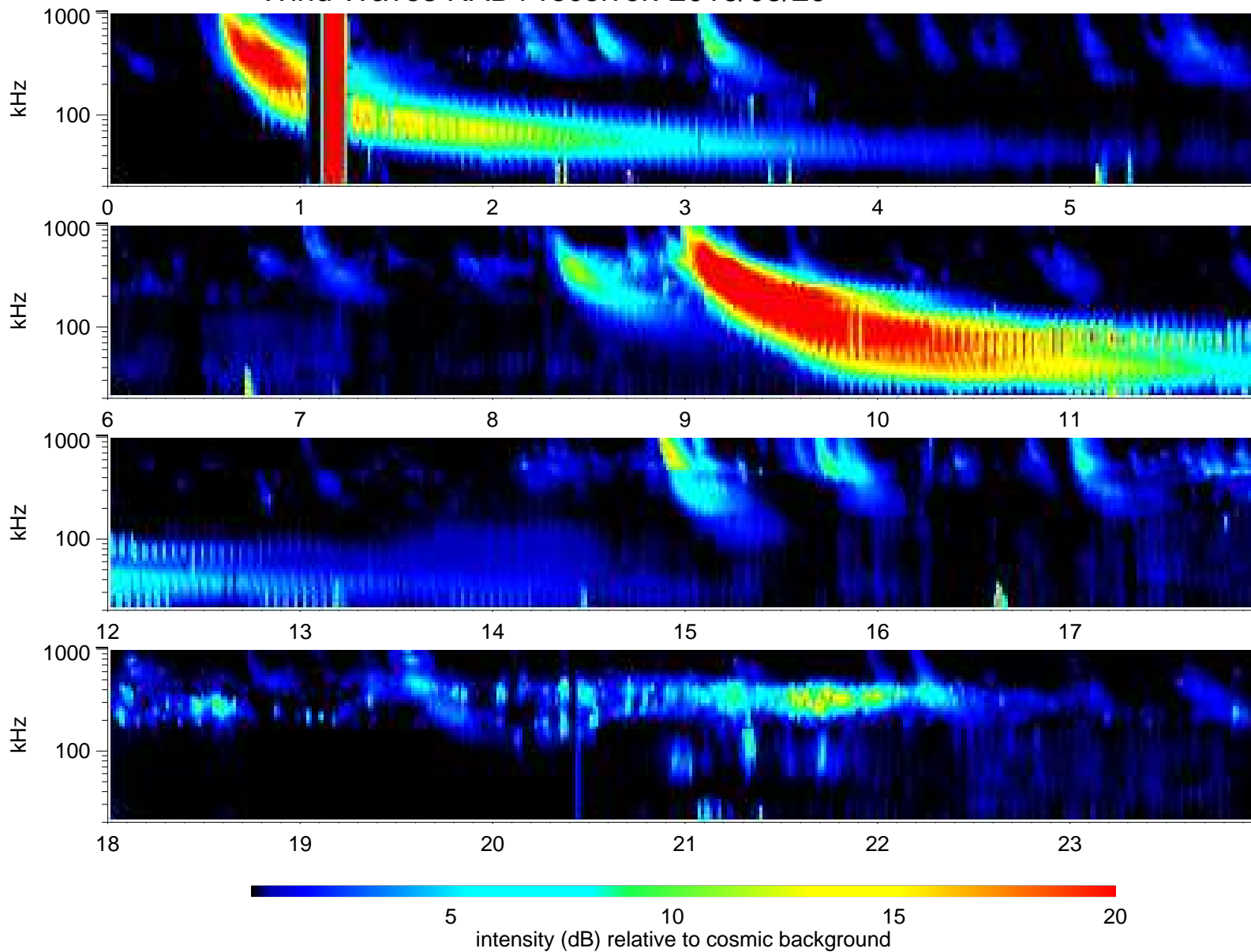
Wind Waves RAD1 receiver: 2016/05/29
