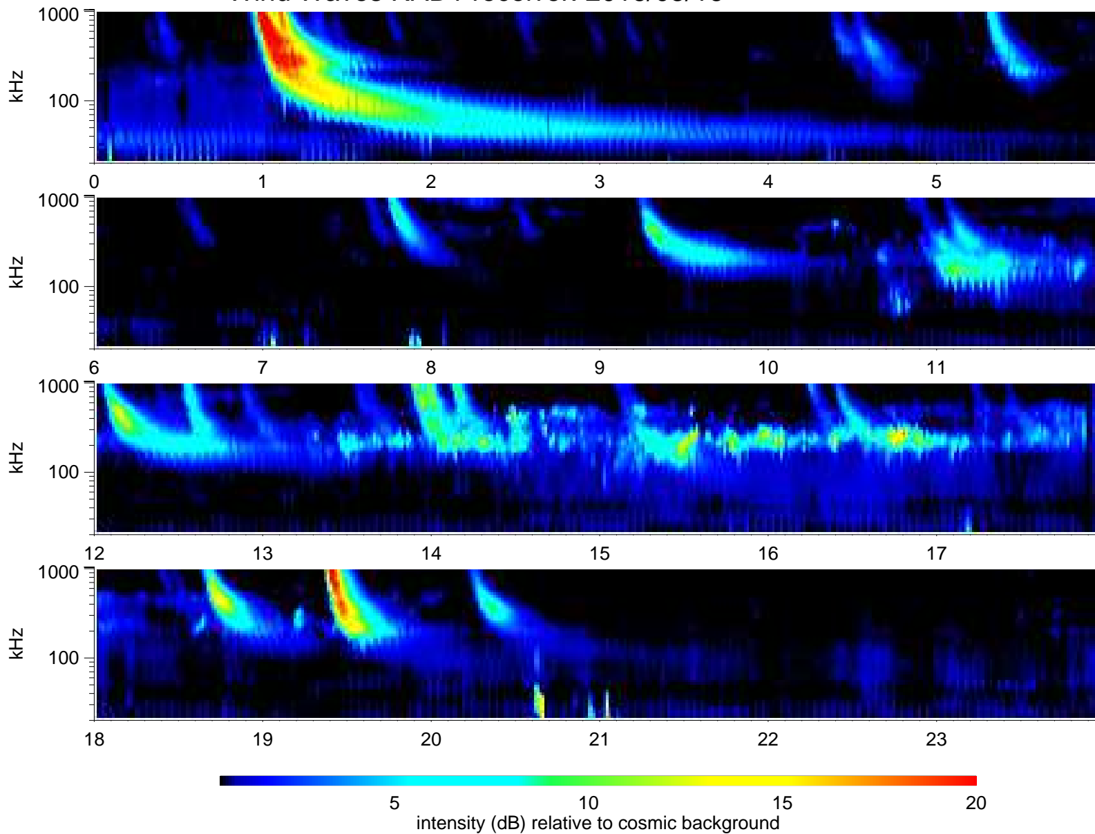
Wind Waves RAD1 receiver: 2016/05/16
