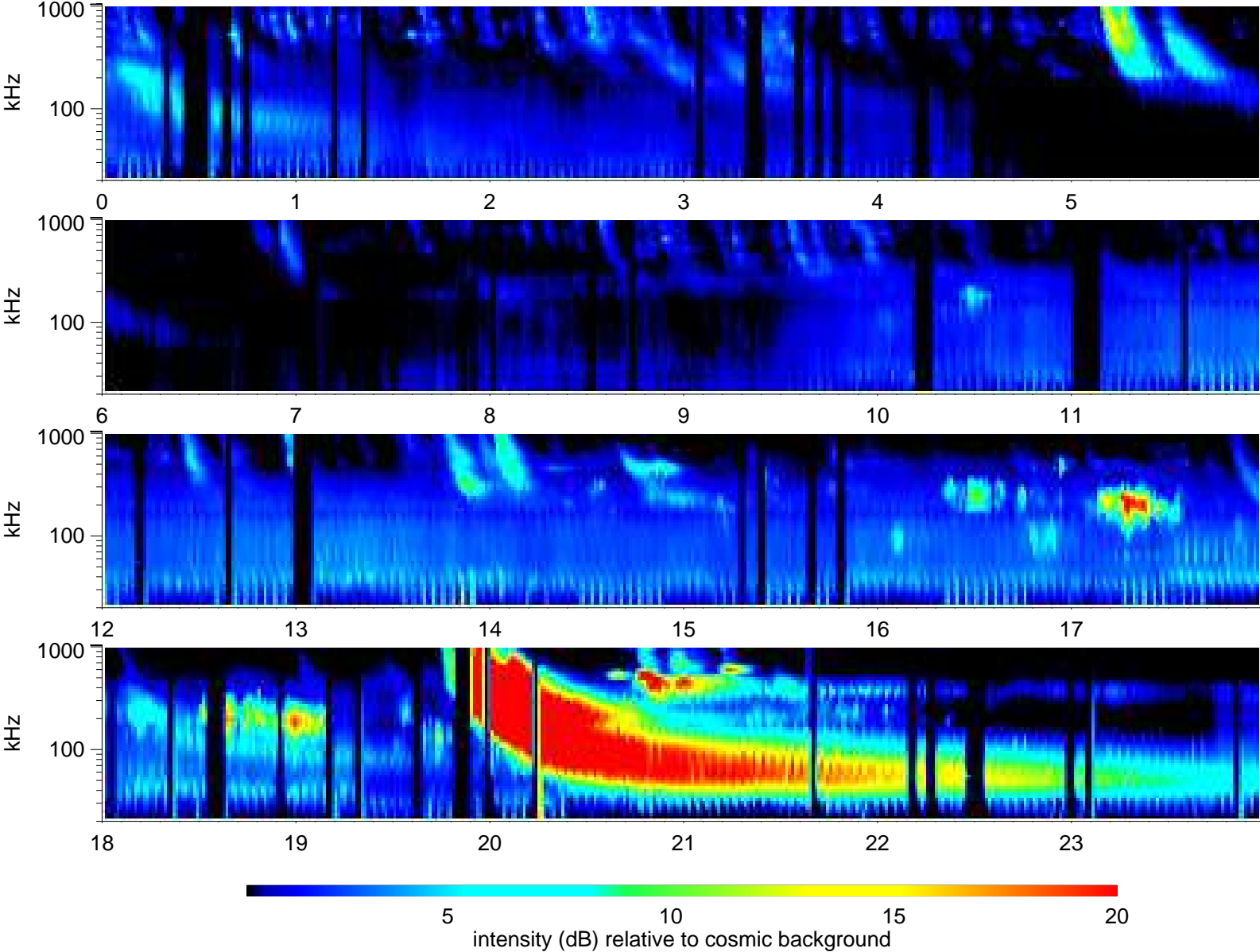
Wind Waves RAD1 receiver: 2016/04/16
