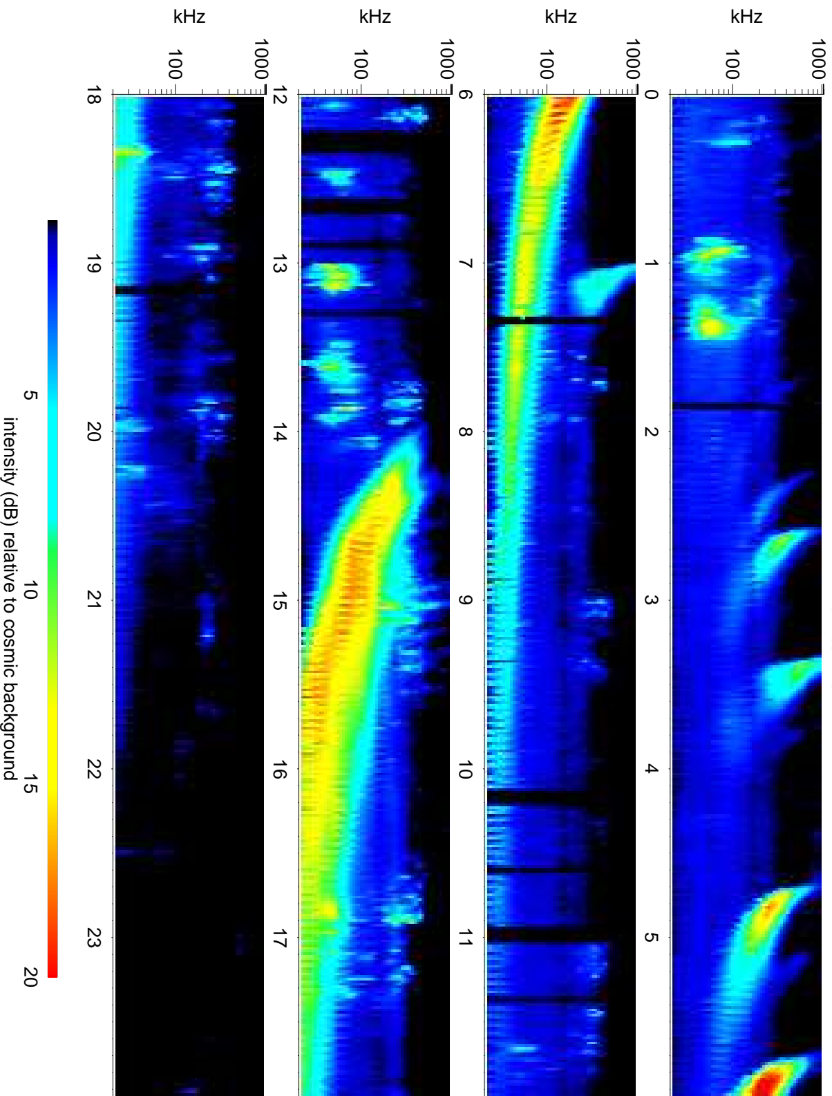
Wind Waves RAD1 receiver: 2015/11/11
