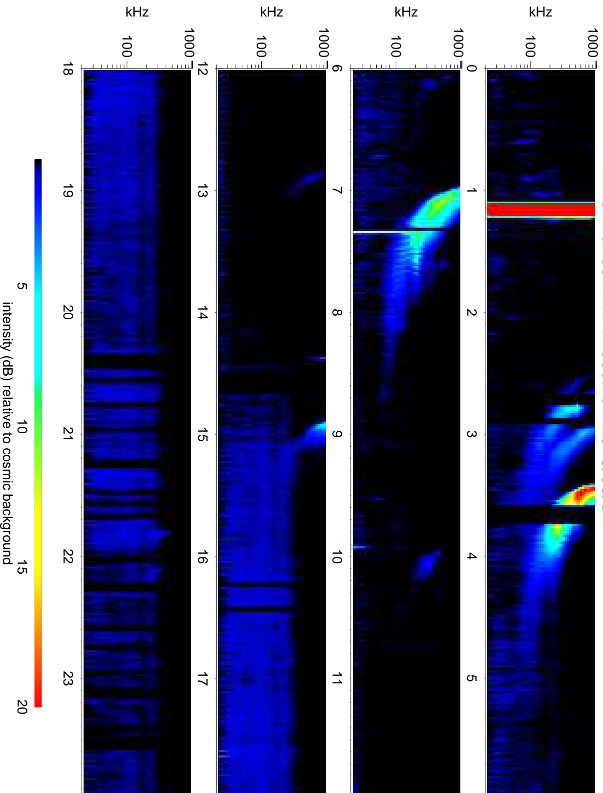
Wind Waves RAD1 receiver: 2015/09/01
