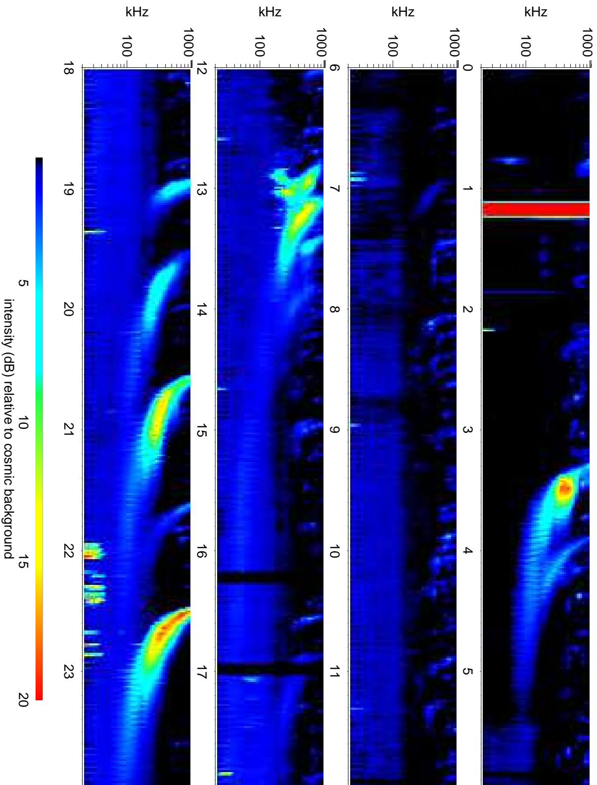
Wind Waves RAD1 receiver: 2014/10/25
