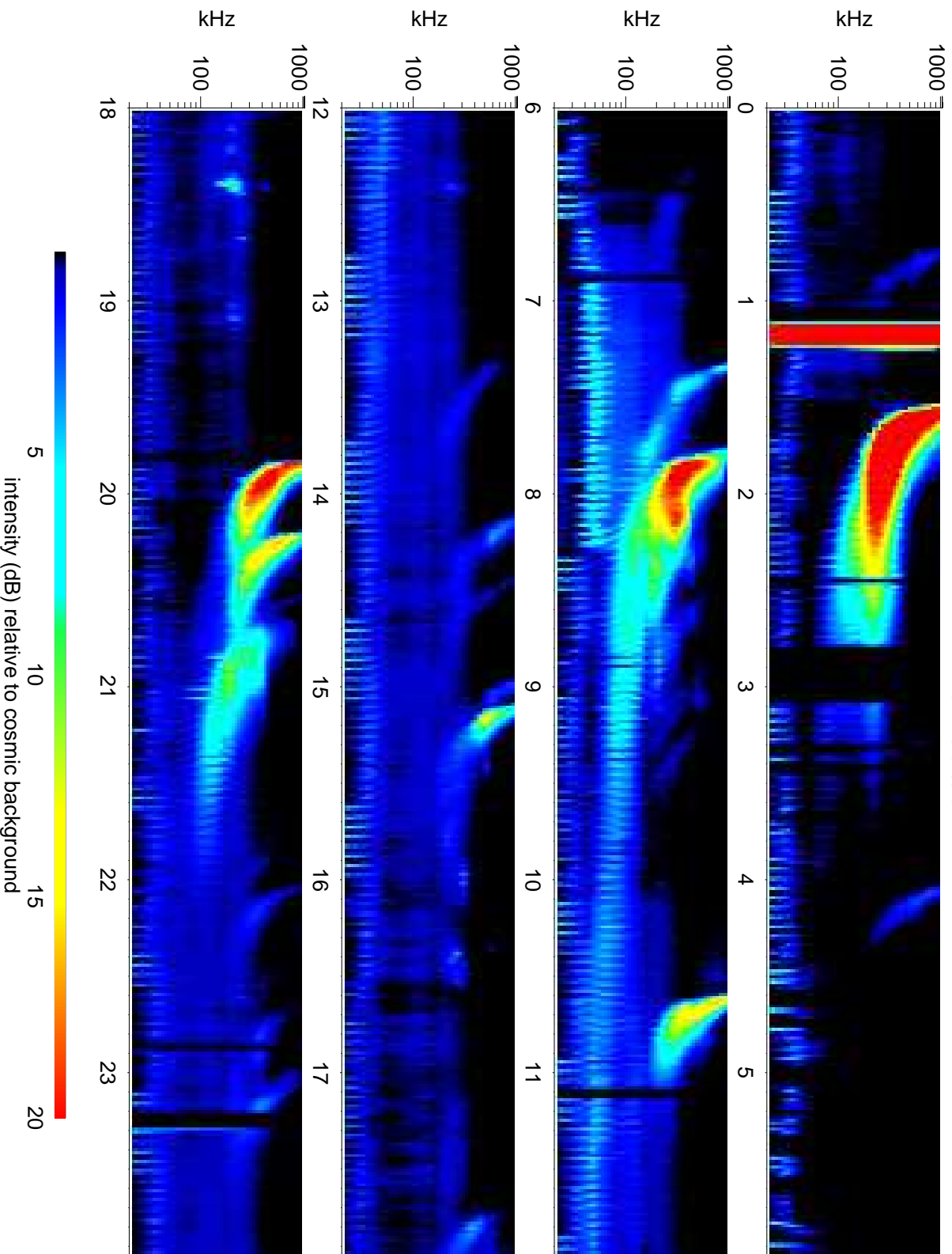
Wind Waves RAD1 receiver: 2014/06/01
