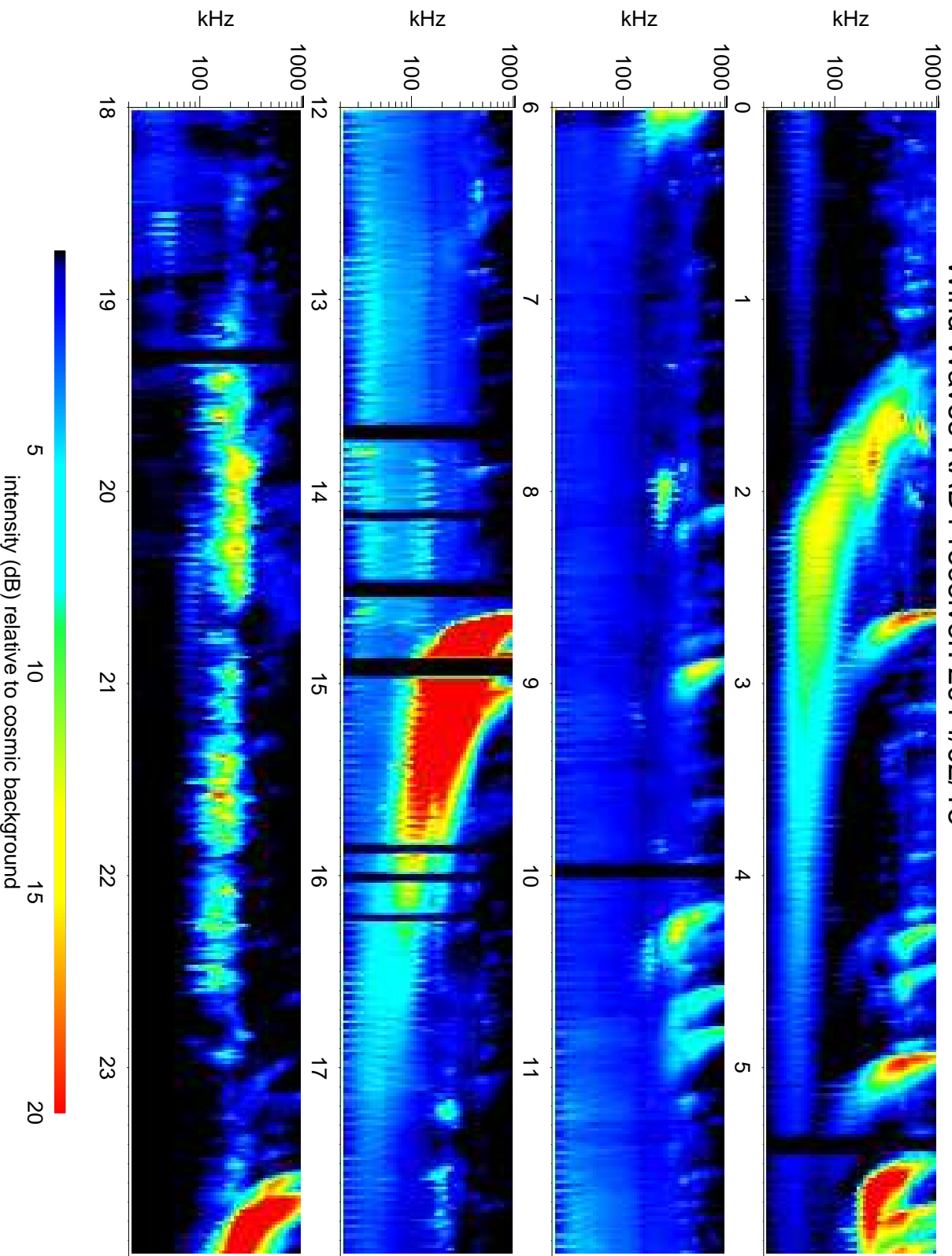
Wind Waves RAD1 receiver: 2014/02/18
