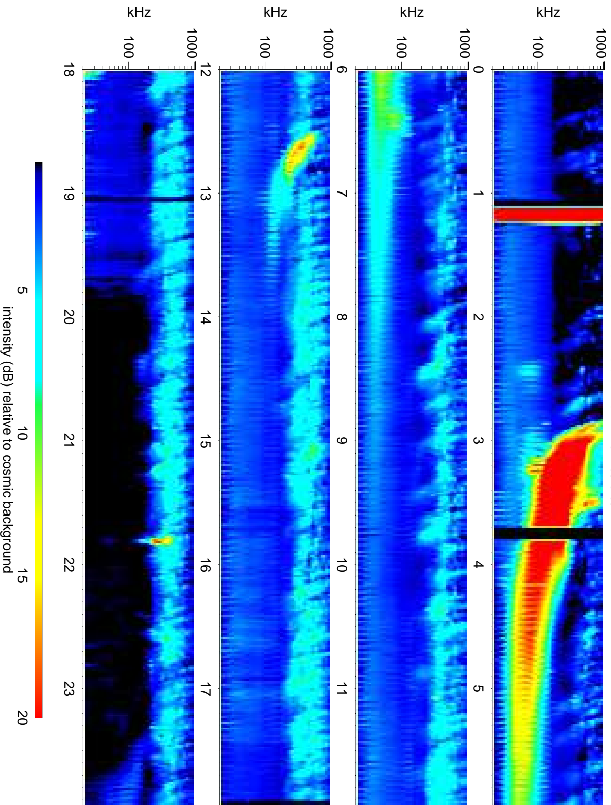
Wind Waves RAD1 receiver: 2013/06/21
